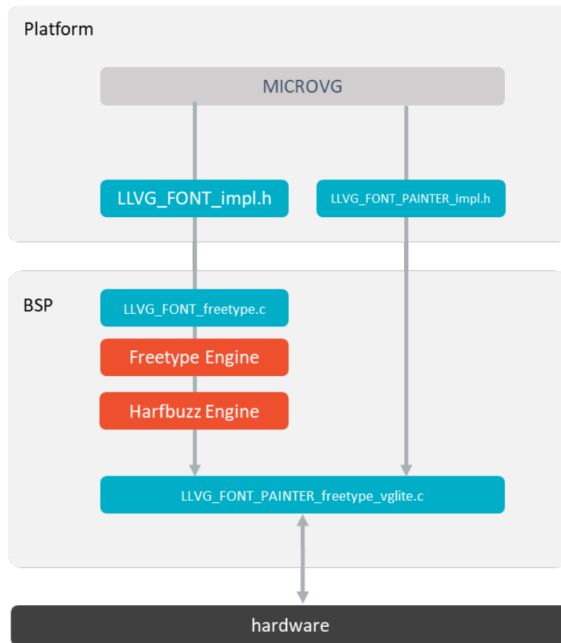
Fig. 53: Font Low-Level API
