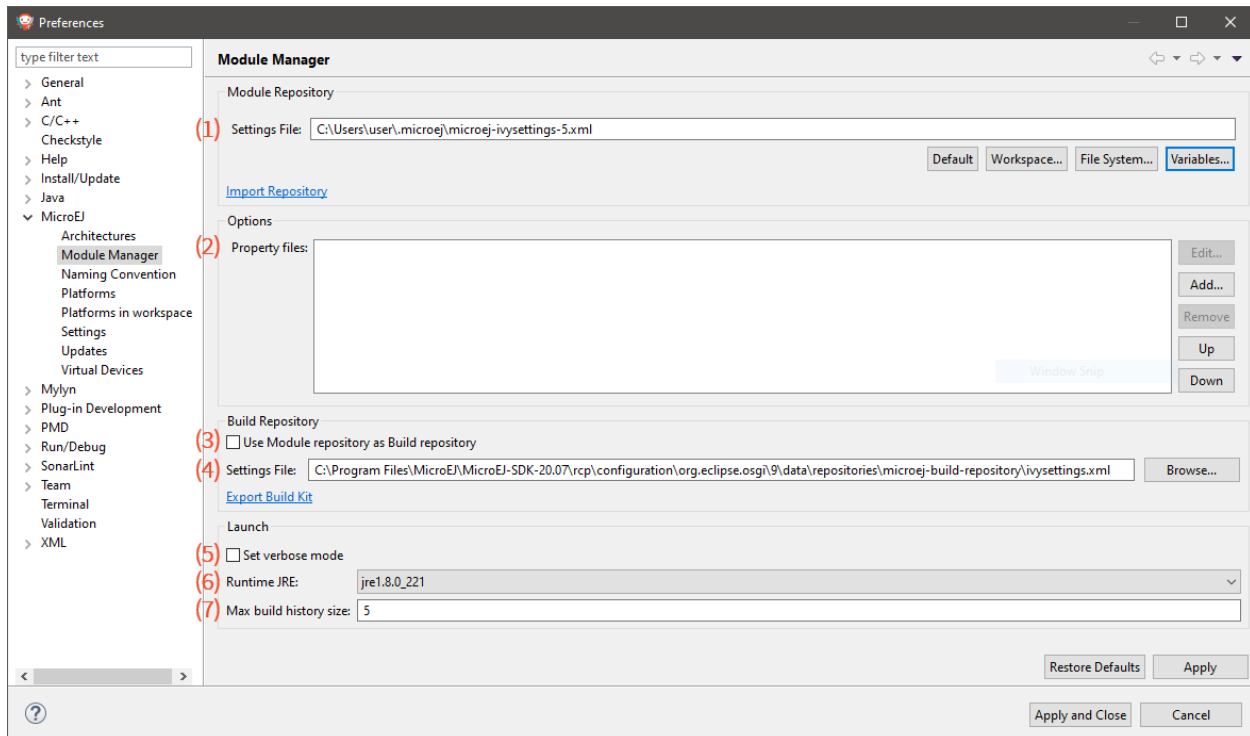
Fig. 34: MMM Preferences Page
