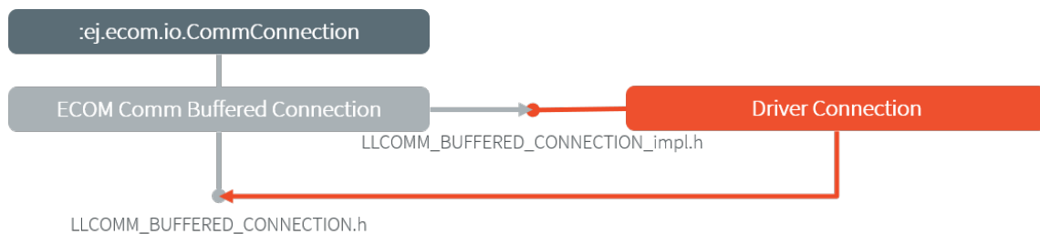
Fig. 28: ECOM Comm components
