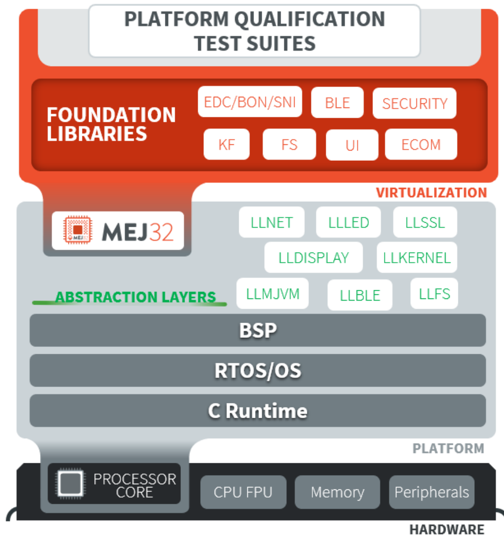
Fig. 16: Platform Qualification Overview
