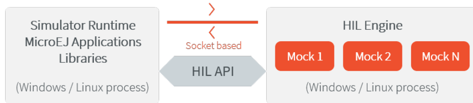
Fig. 51: A MicroEJ Simulator connected to its HIL Engine via a socket.
