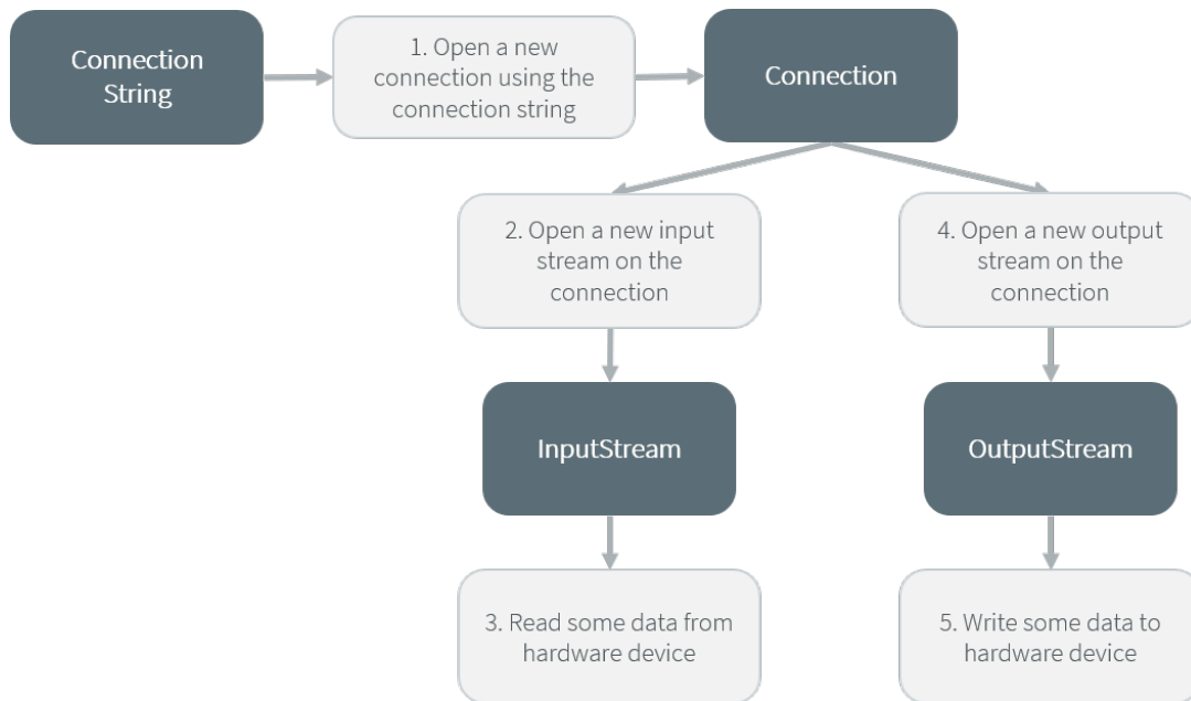
Fig. 27: ECOM Flow
