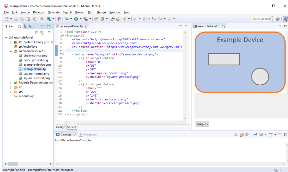
Fig. 57: Working Layout Example
