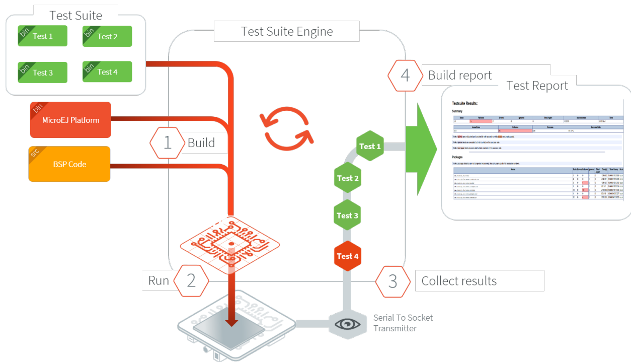
Fig. 18: Platform Test Suite on Device Overview
