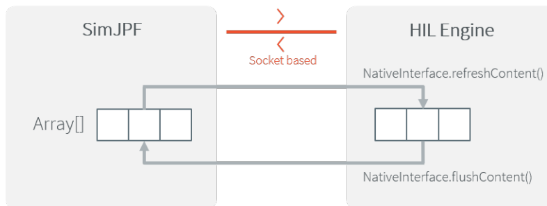
Fig. 53: An Array and Its Counterpart in the HIL Engine.
