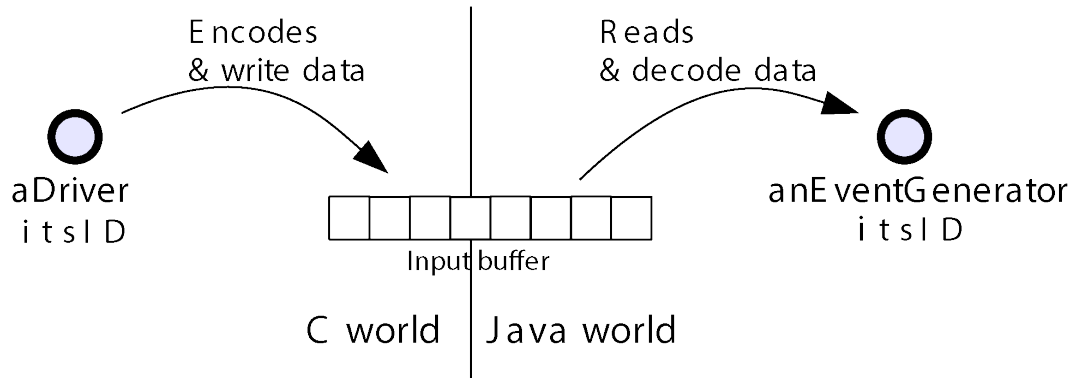
Fig. 38: Drivers and MicroUI Event Generators Communication
