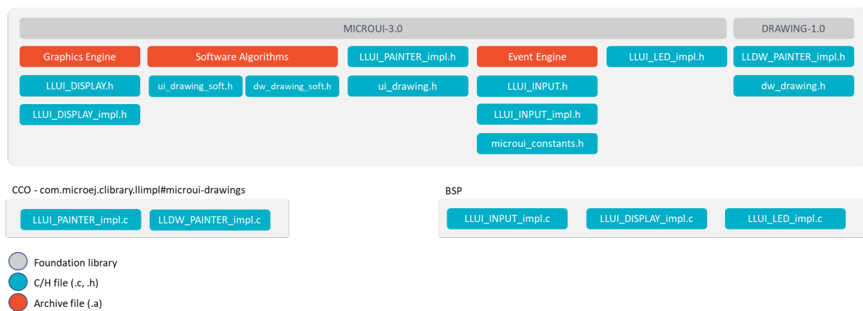
Fig. 35: MicroUI Embedded Low Level API
