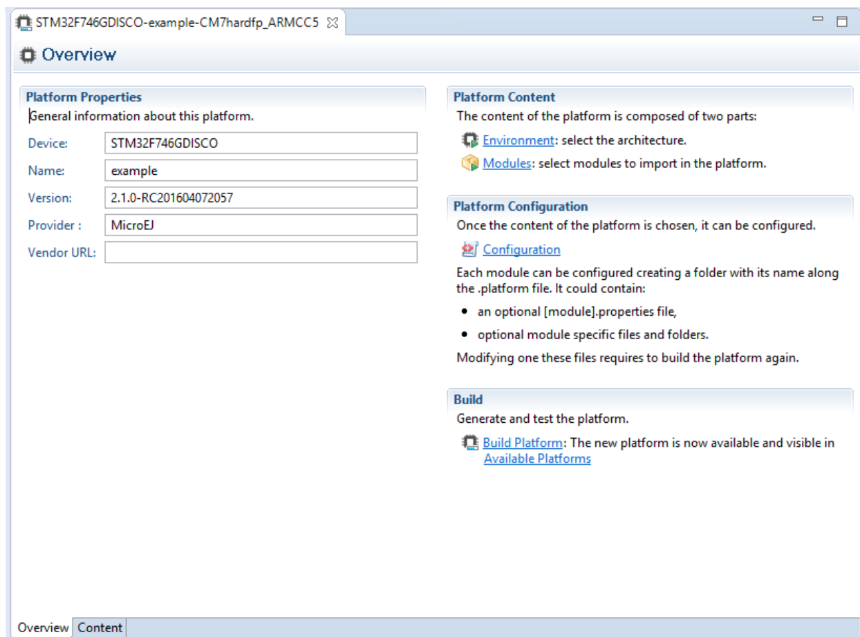
Fig. 3: MicroEJ Platform Configuration Overview Tab
