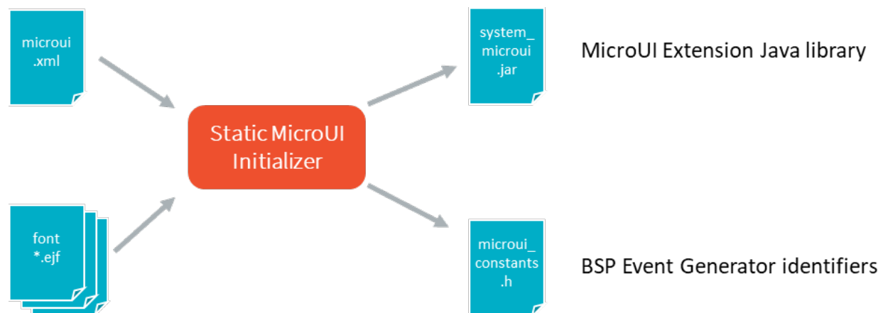
Fig. 33: Static MicroUI Initializer Process
