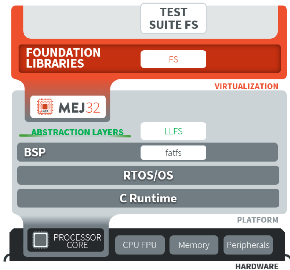
Fig. 17: Platform Qualification Example for FS Pack
