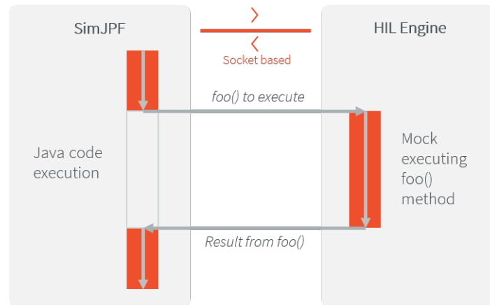
Fig. 52: The MicroEJ Simulator Executes a Native Java Method foo() .
