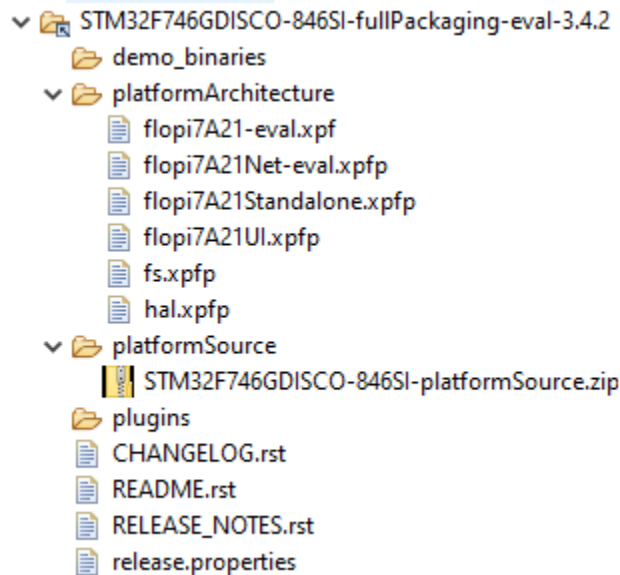
Fig. 14: STM32F746G-DISCO Platform Full Packaging Structure
