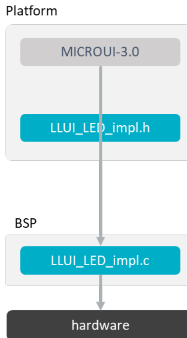
Fig. 37: Led Low Level API
