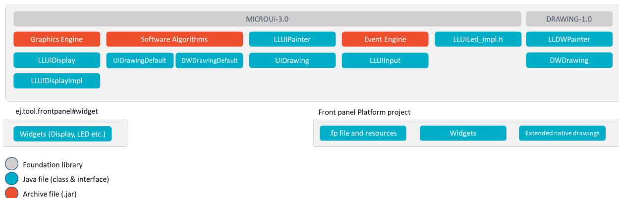
Fig. 36: MicroUI Simulator Low Level API
