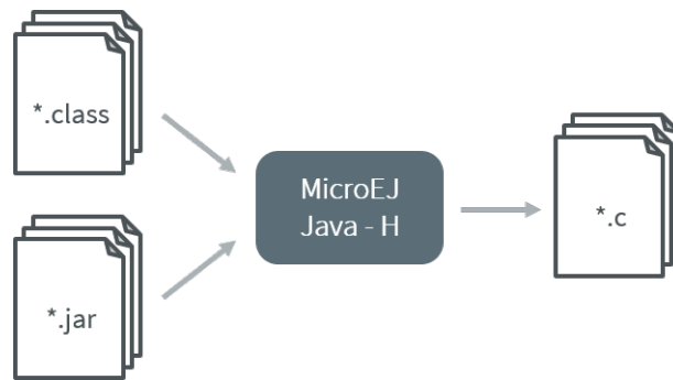
Fig. 26: MicroEJ Java H Process
