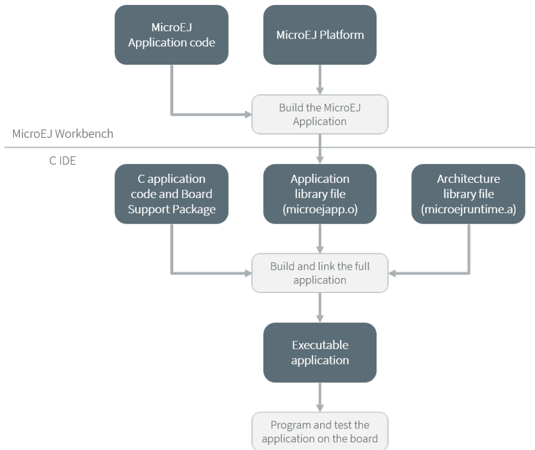
Fig. 19: MicroEJ Core Engine Flow
