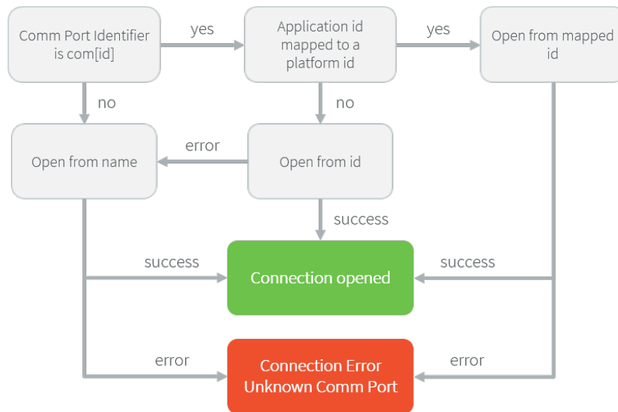
Fig. 29: Comm Port Open Sequence
