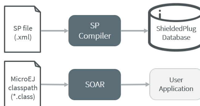
Fig. 25: Shielded Plug Compiler Process Overview
