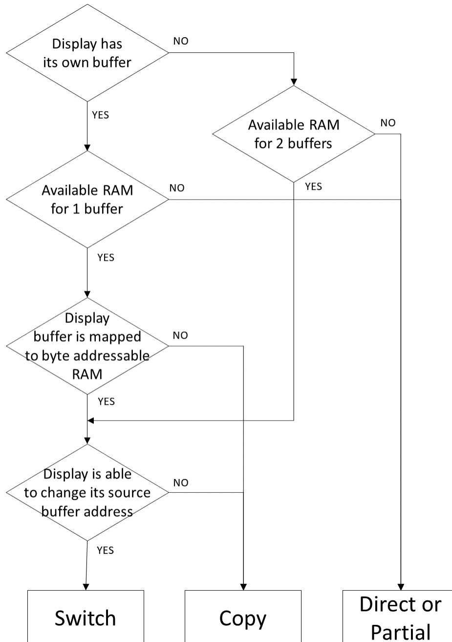
Fig. 41: Buffer Modes
