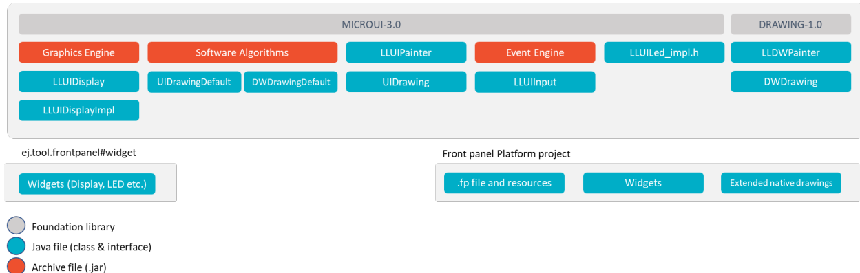
Fig. 36: MicroUI Simulator Low Level API
