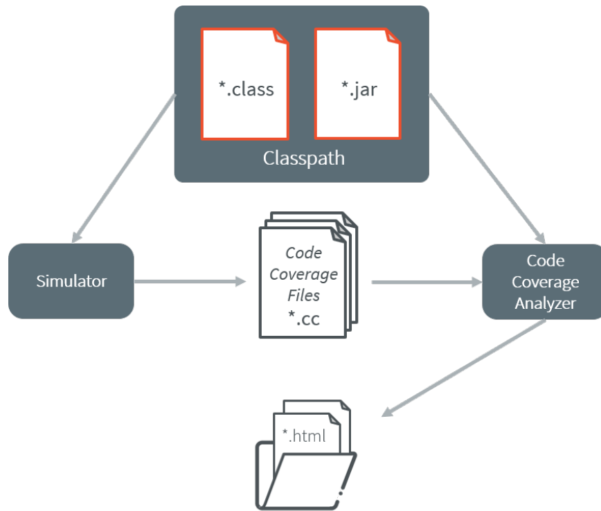
Fig. 41: Code Coverage Analyzer Process
