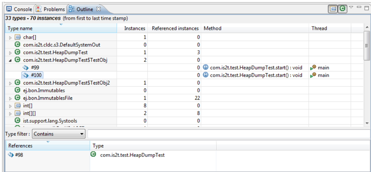
Fig. 42: Outline View
