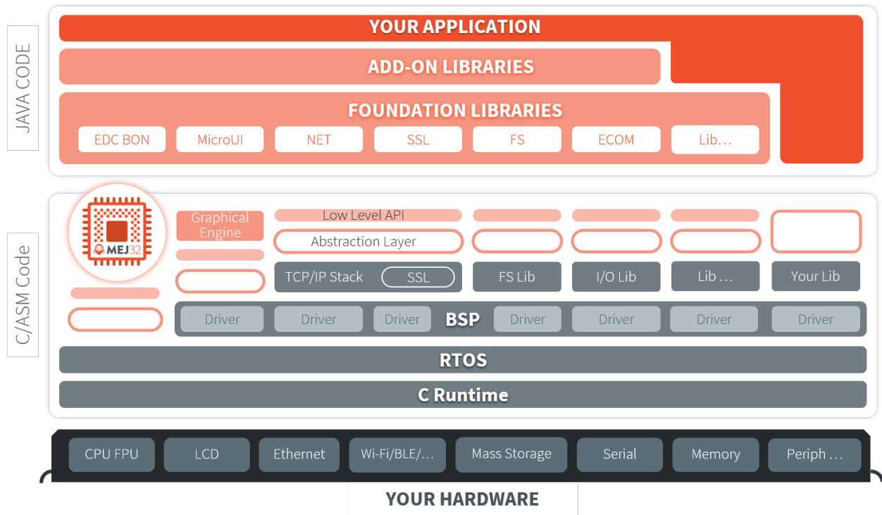
Fig. 10: MicroEJ Firmware Architecture
