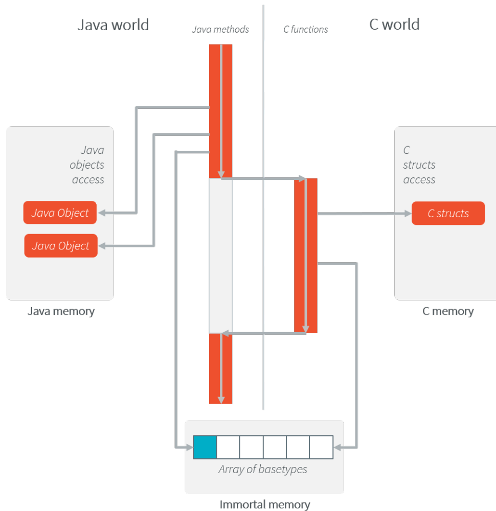
Fig. 20: [SNI] Processing
