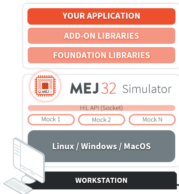
Fig. 46: The HIL Connects the MicroEJ Simulator to the Workstation.
