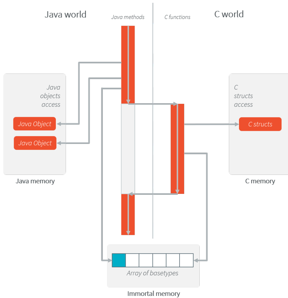
Fig. 18: [SNI] Processing
