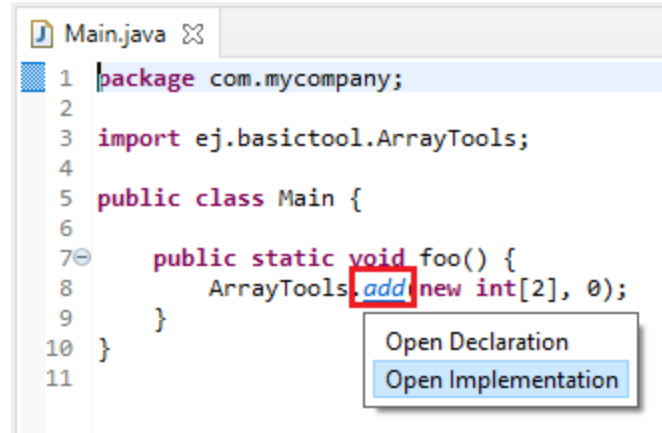
Fig. 27: Add-On Library Open Implementation
