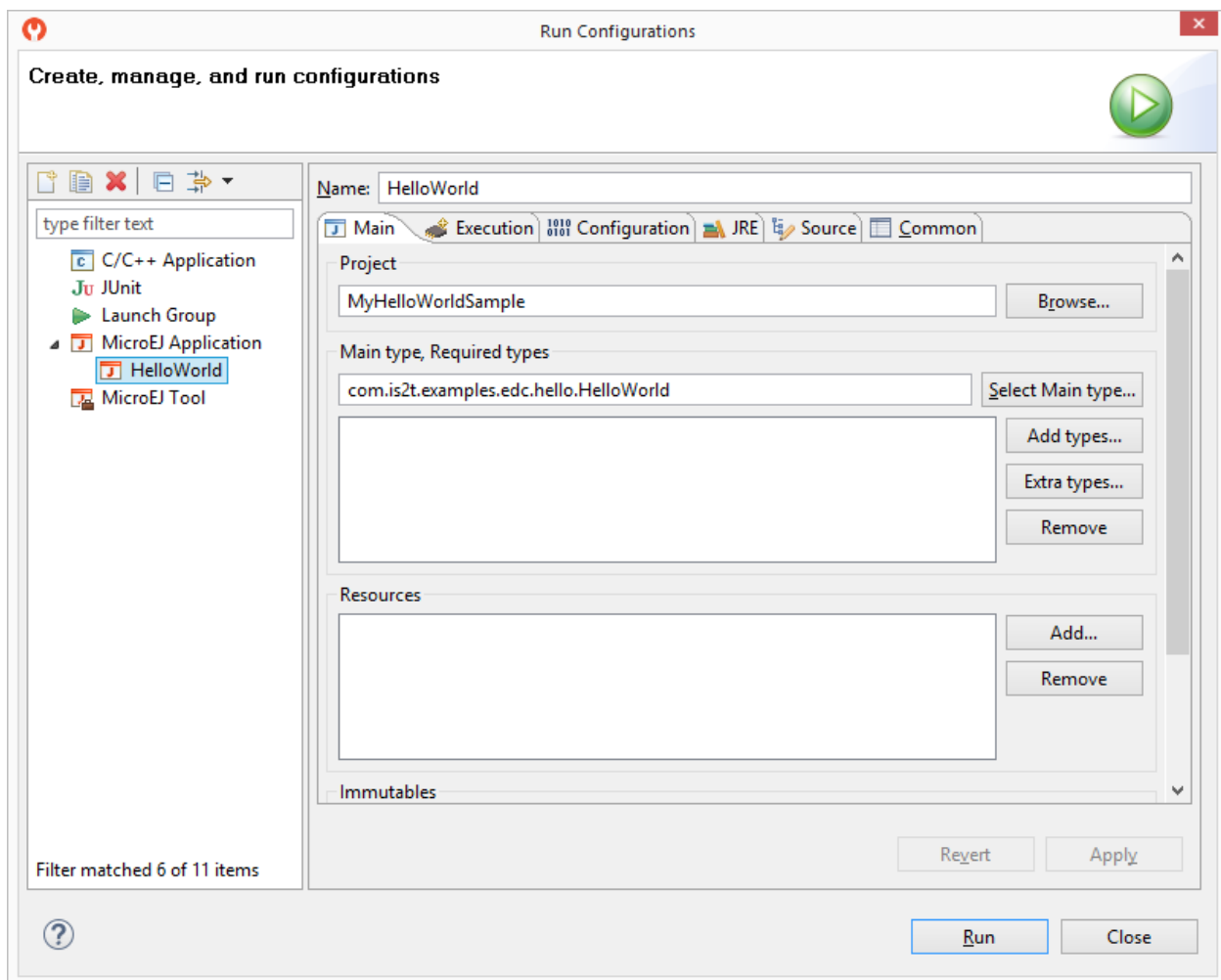
Fig. 12: MicroEJ Launch Application Main Tab
