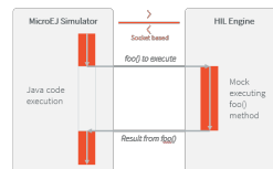
Fig. 59: The MicroEJ Simulator Executes a Native Java Method foo() .
