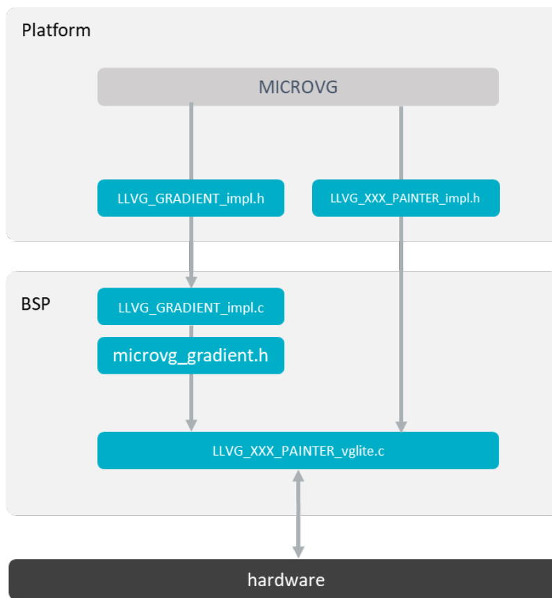
Fig. 52: Gradient Low-Level API
