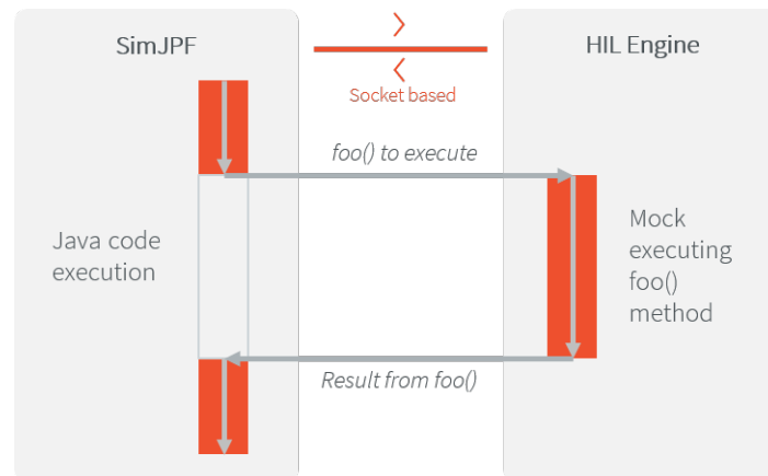
Fig. 46: The MicroEJ Simulator Executes a Native Java Method foo() .
