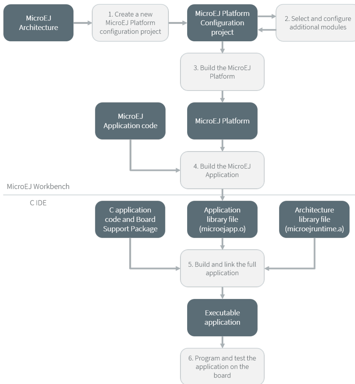
Fig. 2: Overall Process
