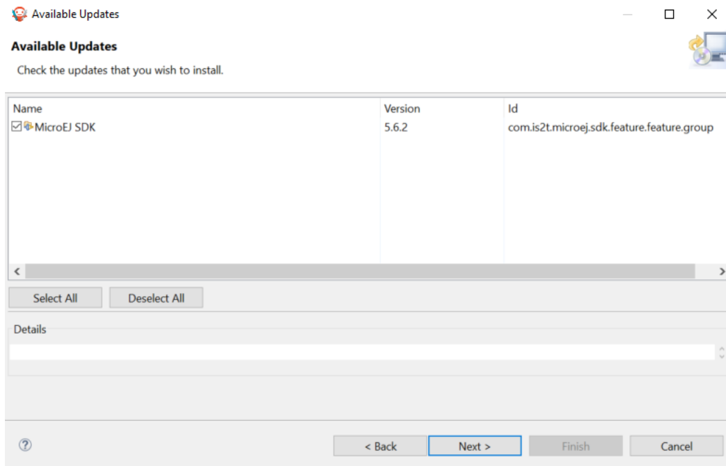
Fig. 12: Update available
