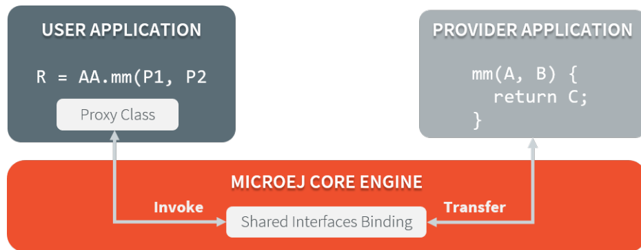
Fig. 15: Shared Interfaces Proxy Overview
