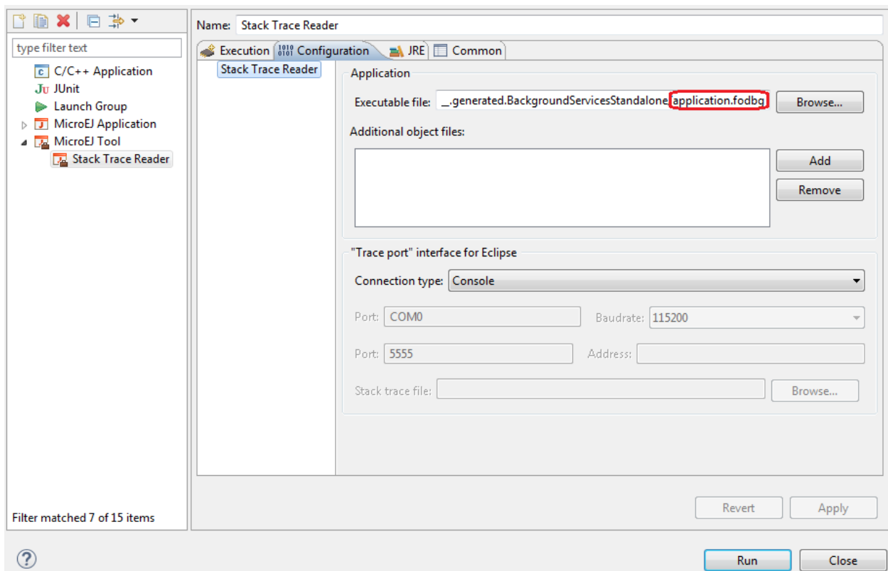
Fig. 36: Stack Trace Reader Tool Configuration (Sandboxed Application)
