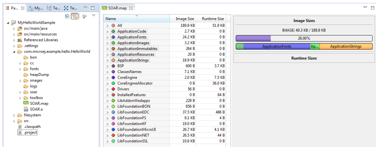
Fig. 57: Consult Full Memory
