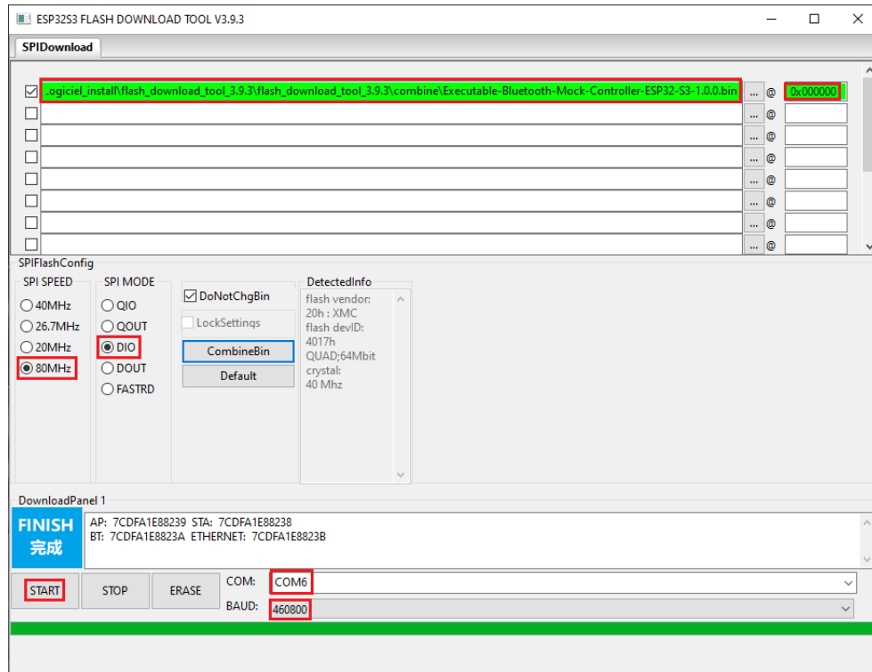
Fig. 67: Bluetooth LE Flash Download Tool Configuration
