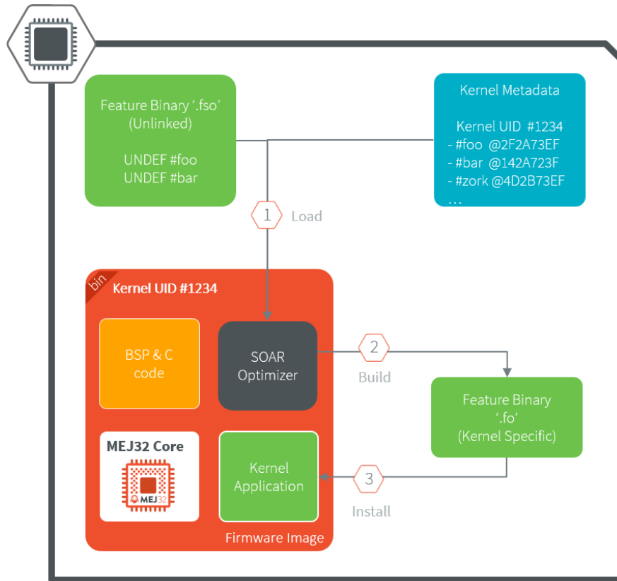
Fig. 14: Sandboxed Application Build on Device
