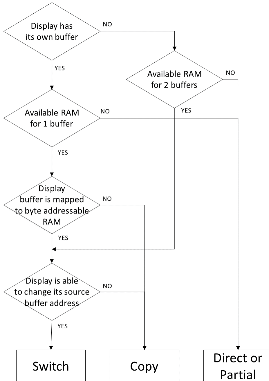
Fig. 39: Buffer Modes
