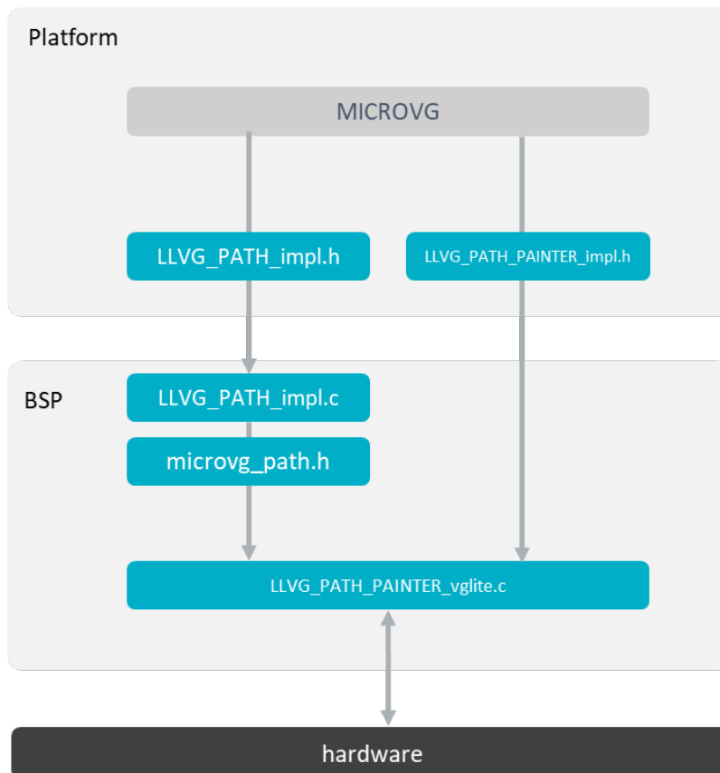
Fig. 51: Path Low-Level API
