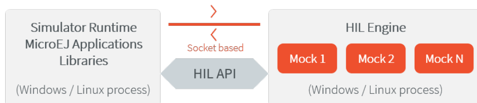
Fig. 58: A MicroEJ Simulator connected to its HIL Engine via a socket.
