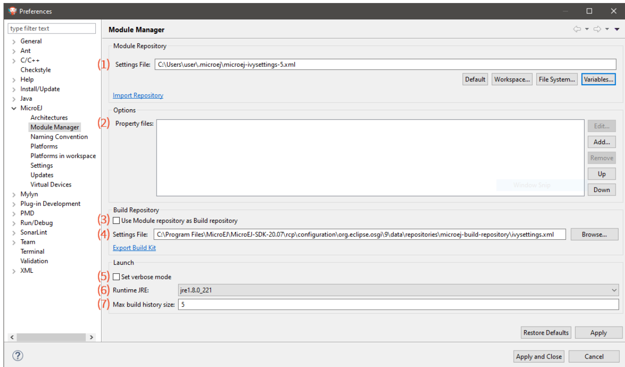
Fig. 18: MMM Preferences Page
