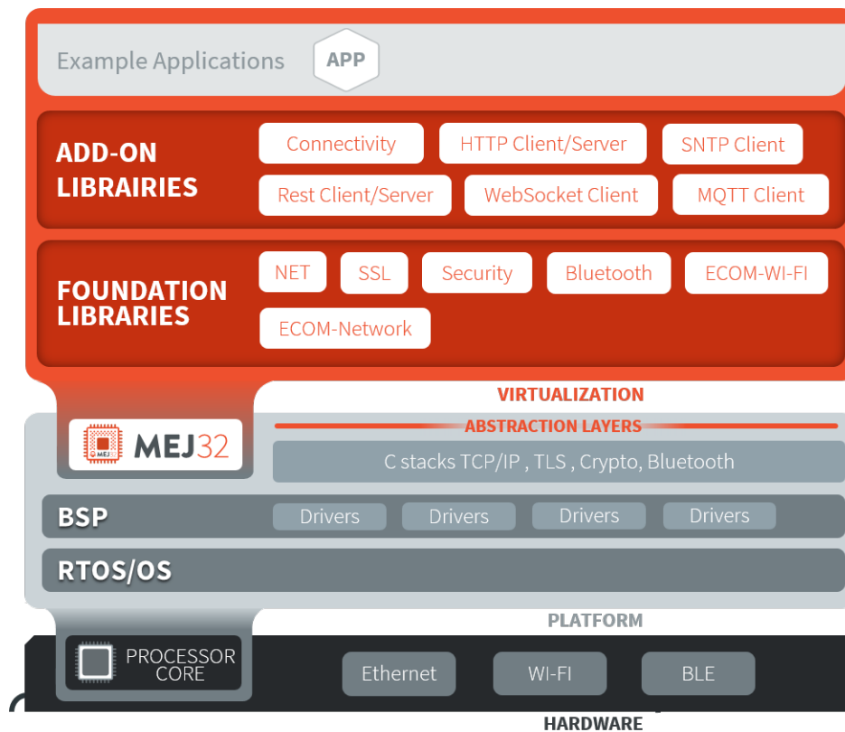
Fig. 85: Network Libraries Overview
