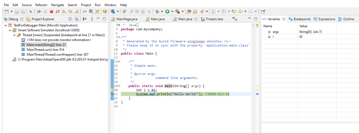
Fig. 31: MicroEJ Development Tools Overview of the Debugger on Simulator
