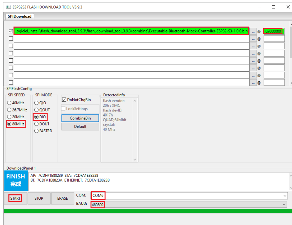
Fig. 75: Bluetooth LE Flash Download Tool Configuration
