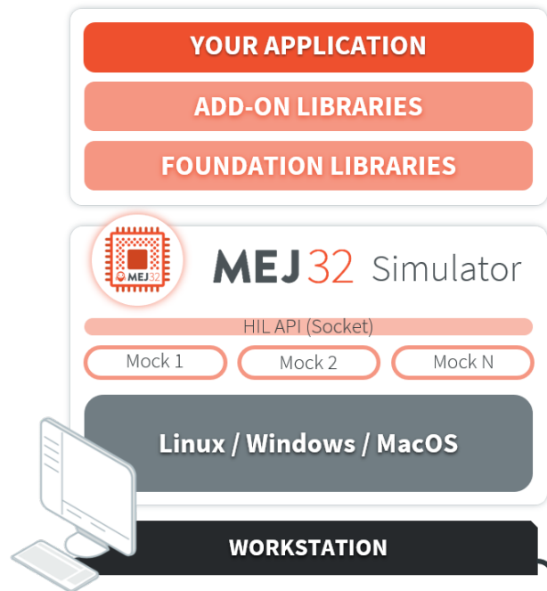
Fig. 65: The HIL Connects the MicroEJ Simulator to the Workstation.
