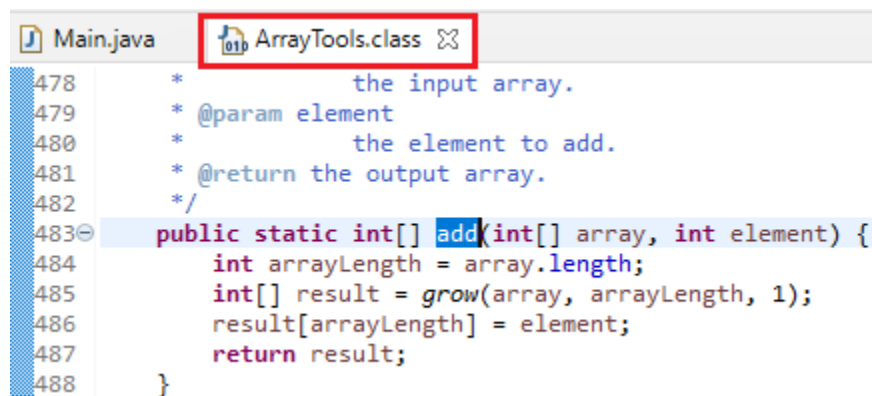
Fig. 36: Add-On Library Read-Only Source Code
