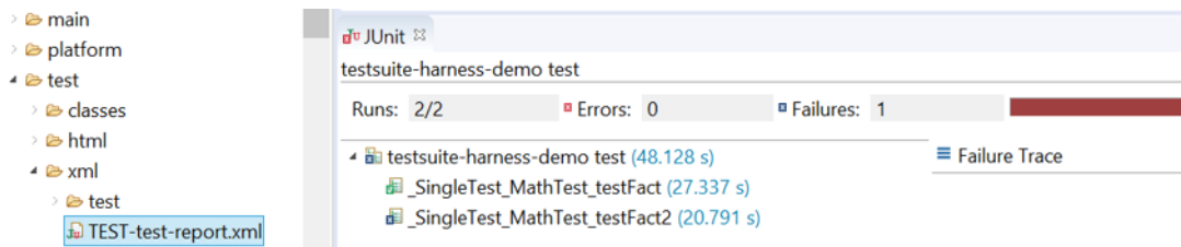
Fig. 44: Example of MicroEJ Test Suite XML Report in JUnit View
