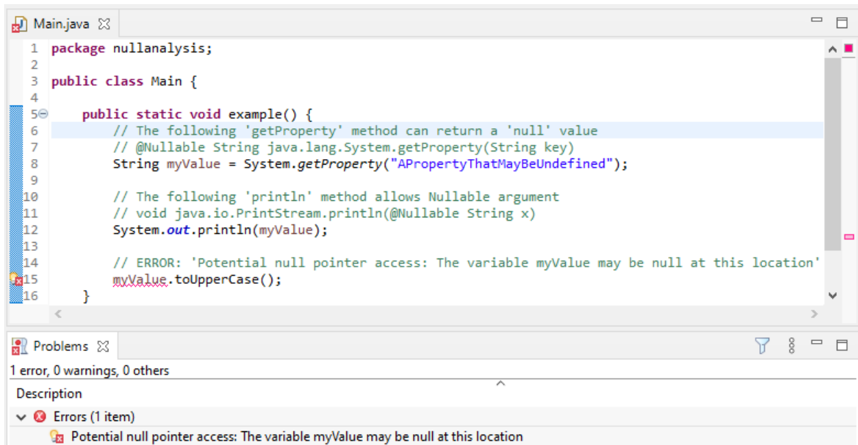
Fig. 74: Example of Null Analysis Detection
