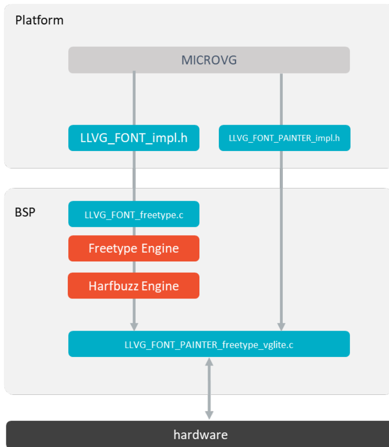
Fig. 61: Font Low-Level API
