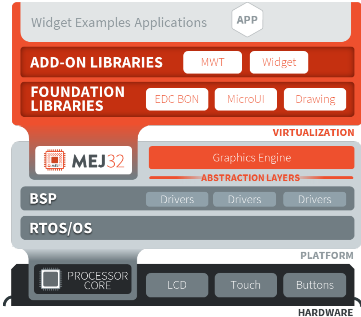
Fig. 77: Graphical User Interface Overview
