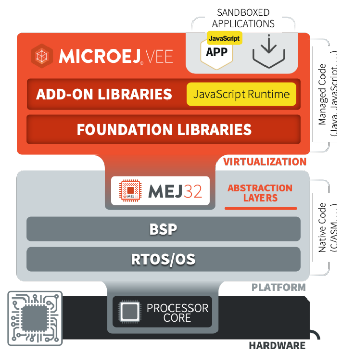
Fig. 84: MicroEJ JavaScript Overview
