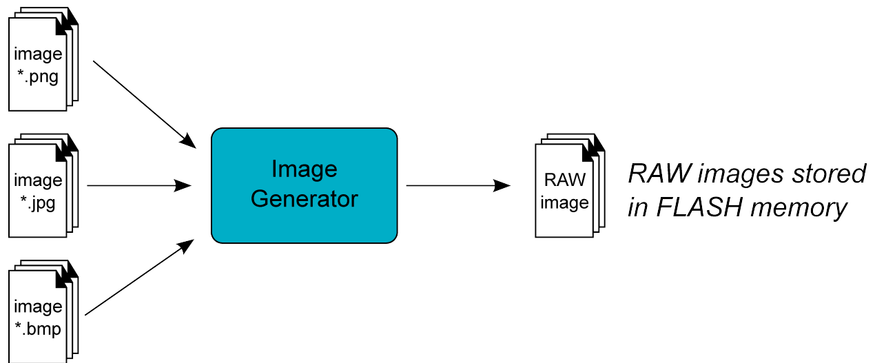
Fig. 49: Image Generator Principle
