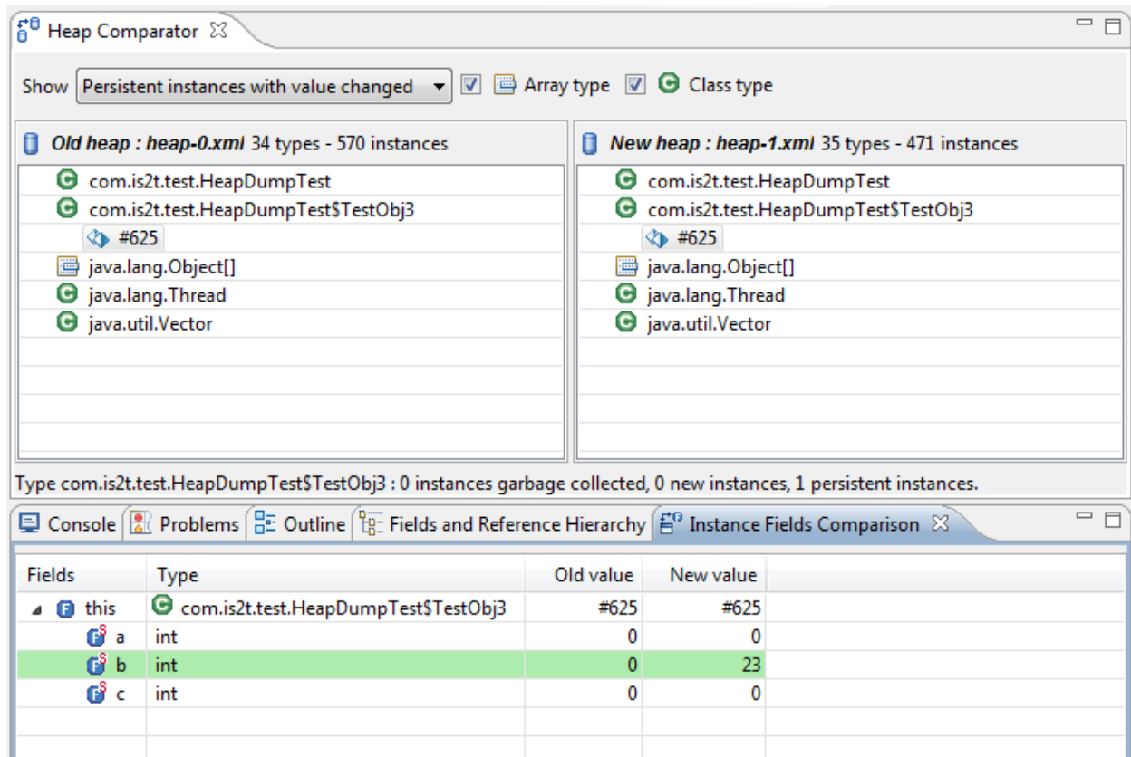
Fig. 69: Instance Fields Comparison view
