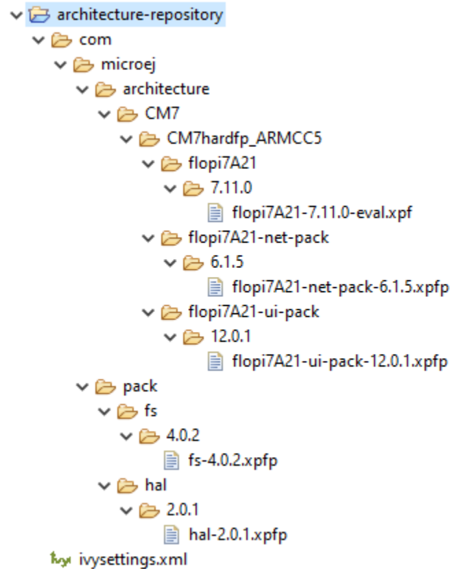
Fig. 78: Architecture Repository for STM32F746G-DISCO fullPackaging
