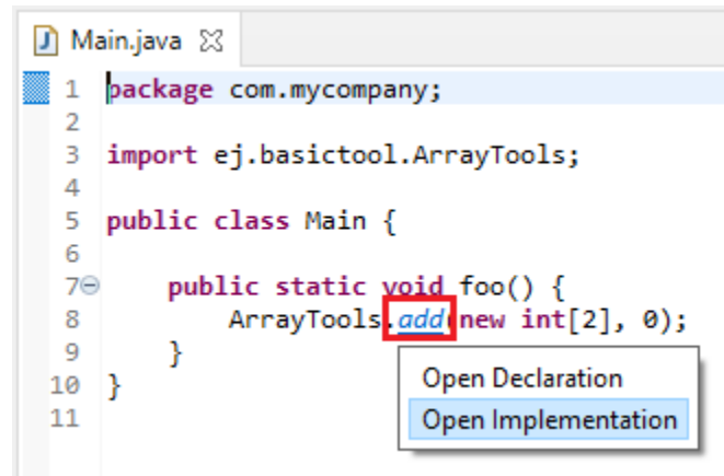
Fig. 35: Add-On Library Open Implementation
