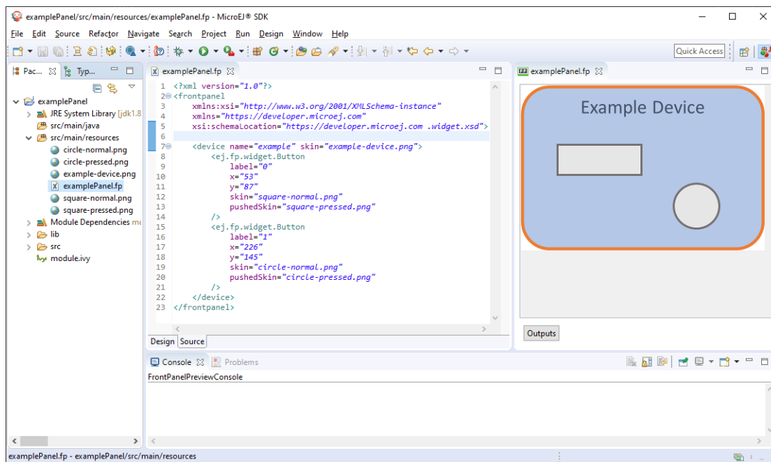
Fig. 72: Working Layout Example
