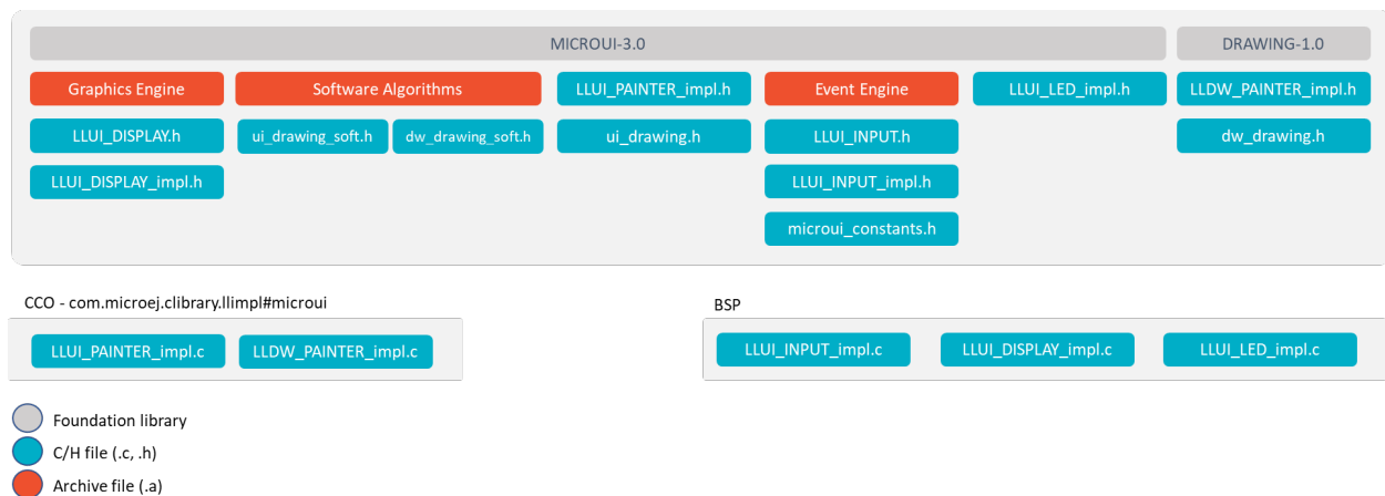
Fig. 41: MicroUI Embedded Low Level API
