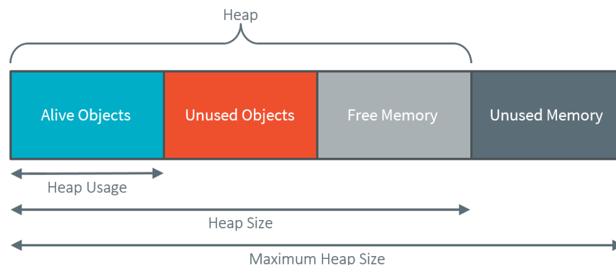
Fig. 60: Heap Structure Summary
