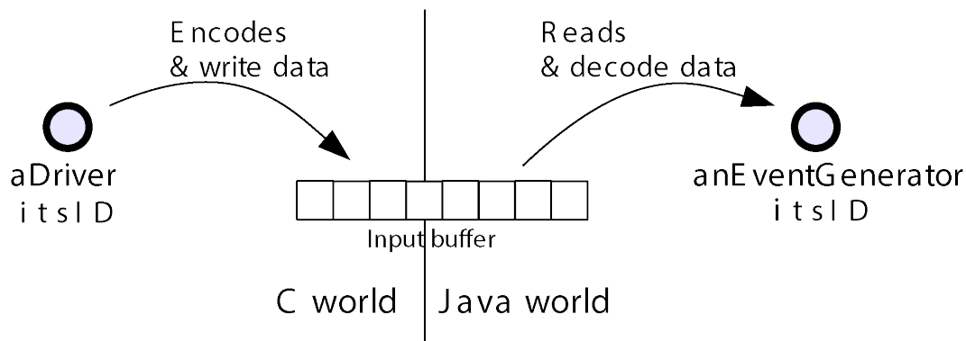
Fig. 44: Drivers and MicroUI Event Generators Communication
