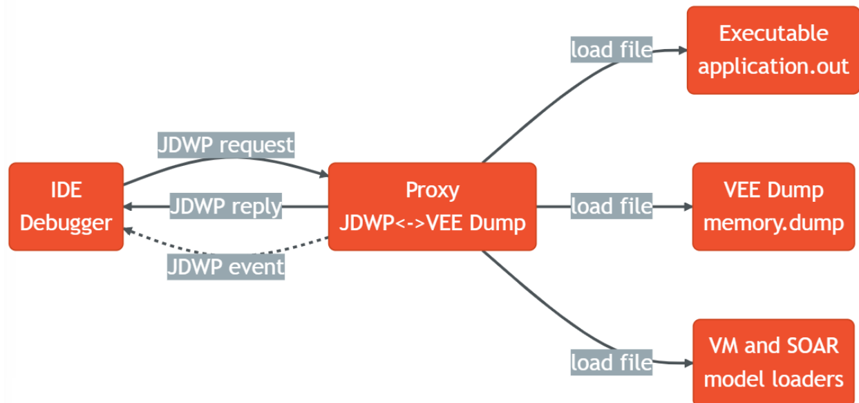
Fig. 76: Debugger Proxy Principle
