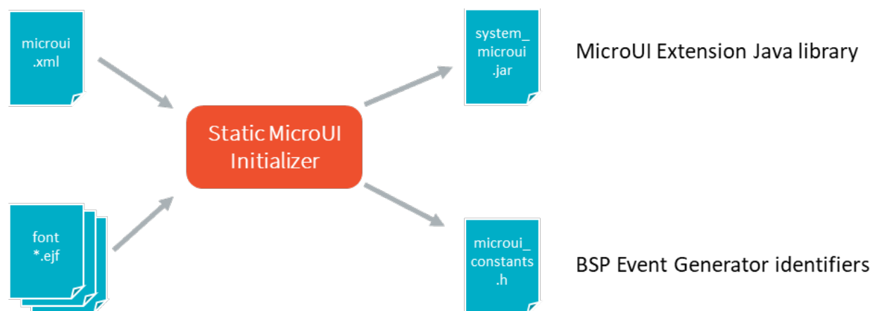
Fig. 39: Static MicroUI Initializer Process
