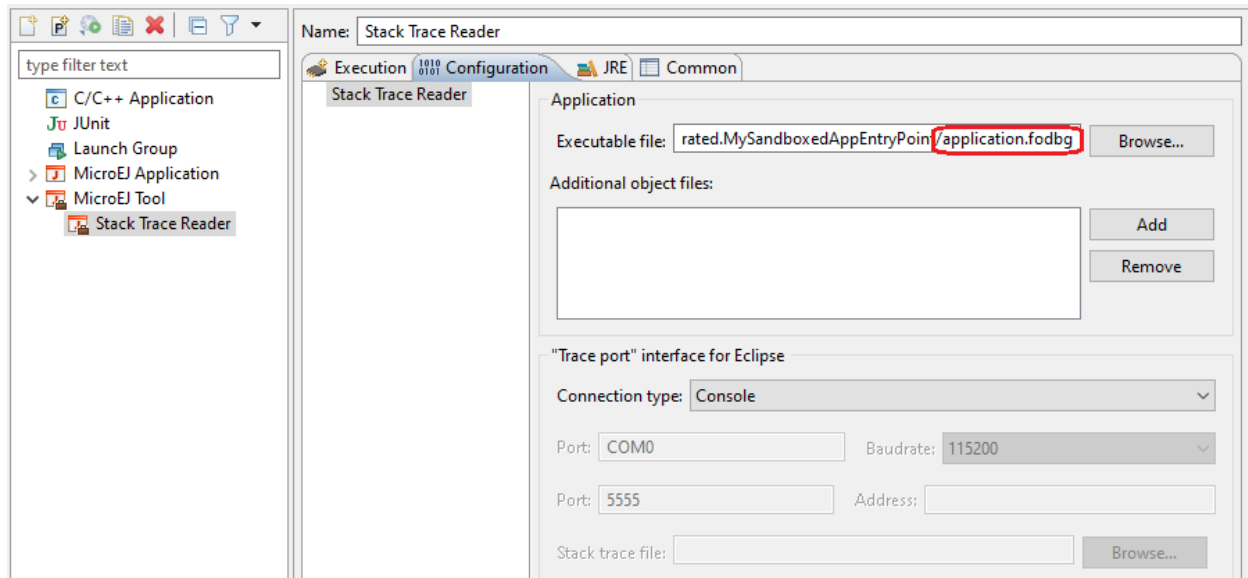
Fig. 57: Stack Trace Reader Tool Configuration (Sandboxed Application)
