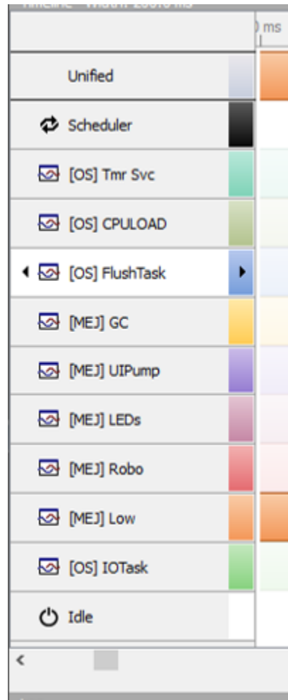
Fig. 64: OS Tasks and Java Threads Names
