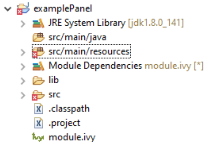
Fig. 55: Project Contents
