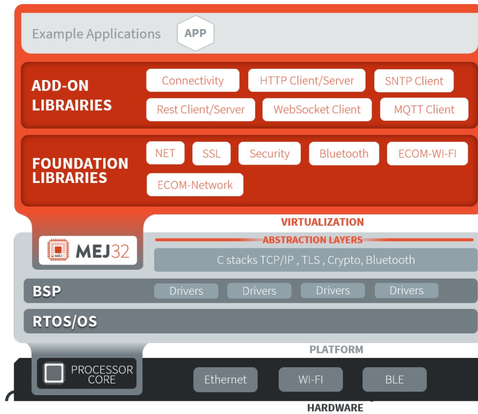
Fig. 76: Network Libraries Overview
