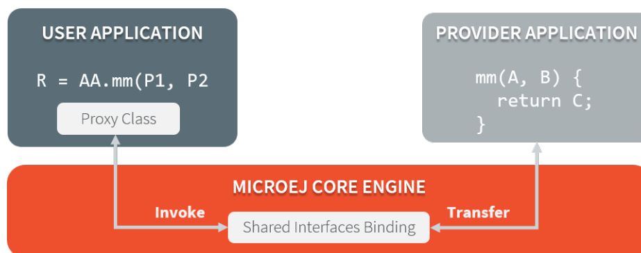
Fig. 22: Shared Interfaces Proxy Overview
