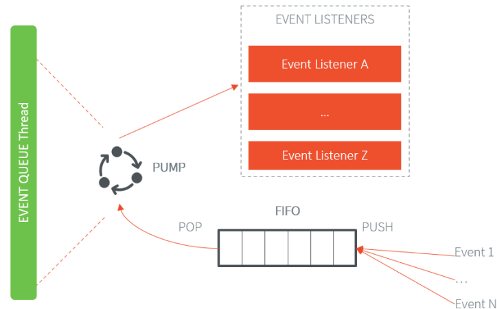
Fig. 95: Event Queue Overview
