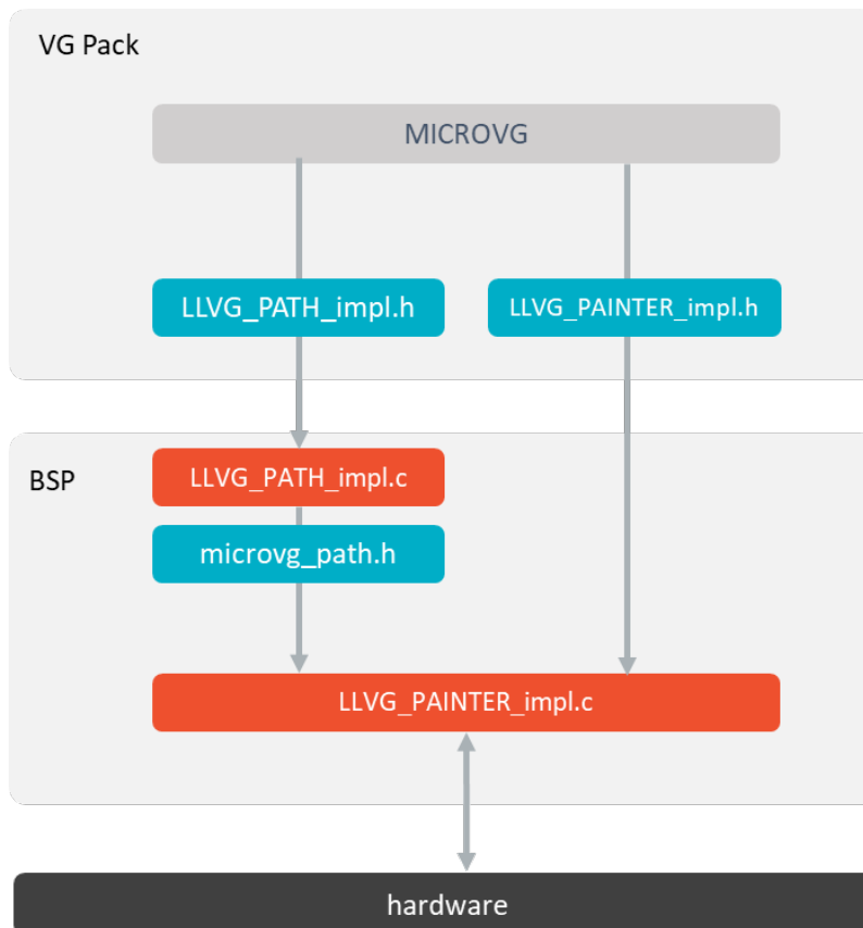
Fig. 61: Path Abstraction Layer API
