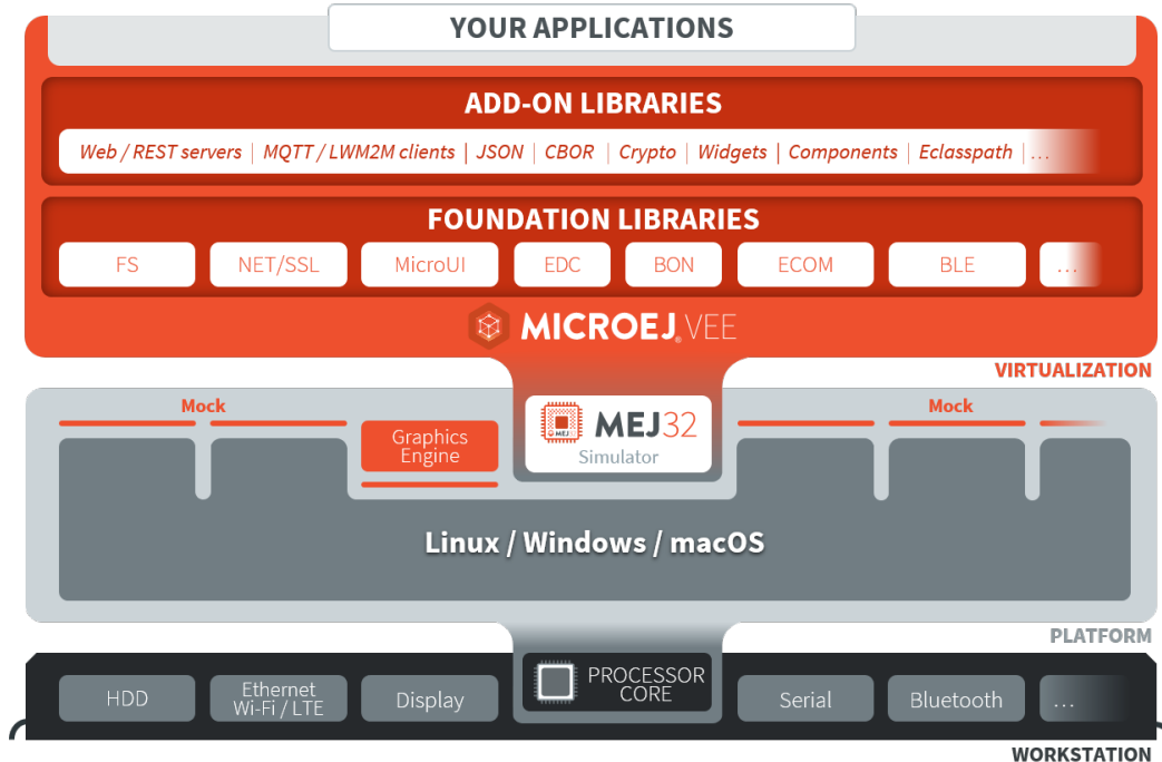
Fig. 26: MicroEJ Virtual Device Architecture
