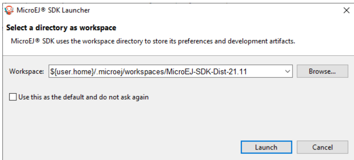
Fig. 12: Workspace selection
