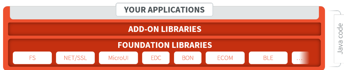
Fig. 19: MicroEJ Foundation Libraries and Add-On Libraries
