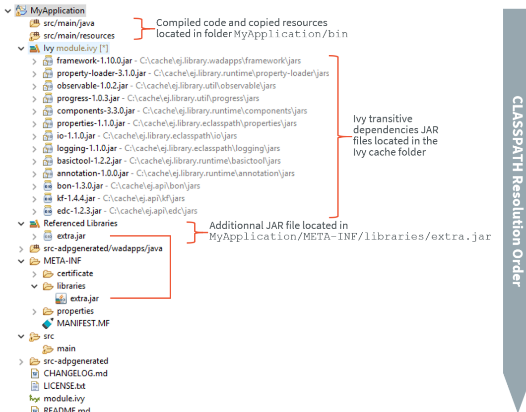
Fig. 24: MicroEJ Application Classpath Mapping
