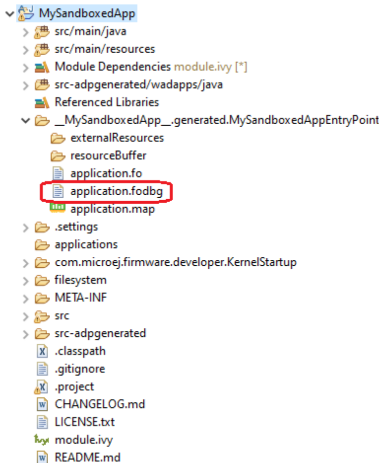
Fig. 45: Application Binary File with Debug Information
