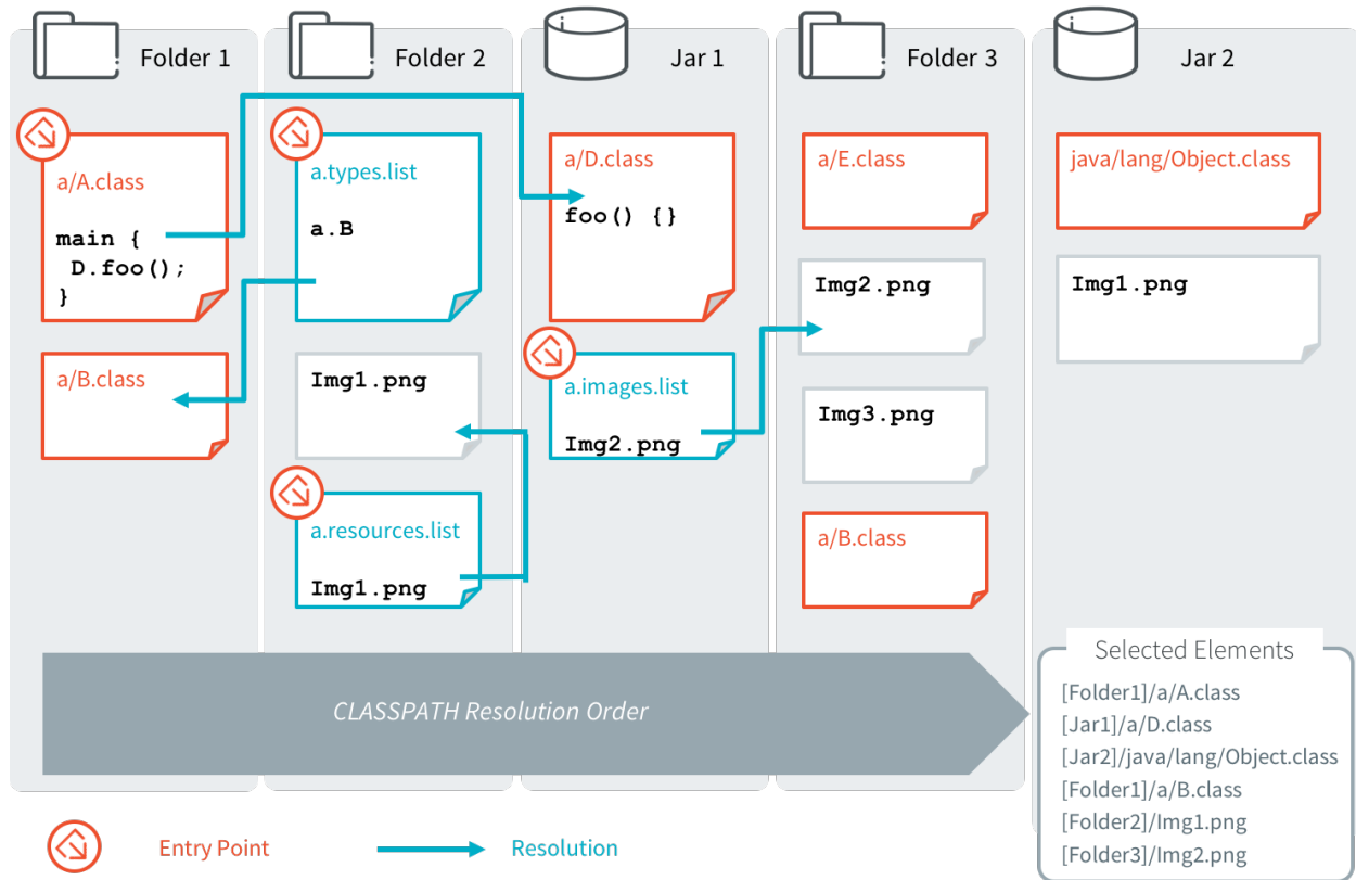
Fig. 25: Classpath Load Principle
