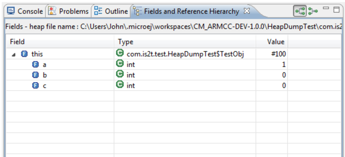
Fig. 55: Instance Browser View - Fields mode
