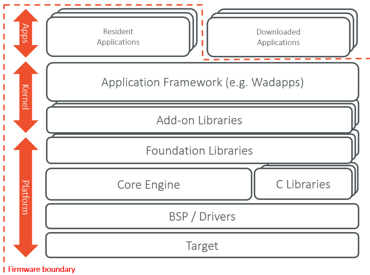
Fig. 1: Firmware Boundary Overview
