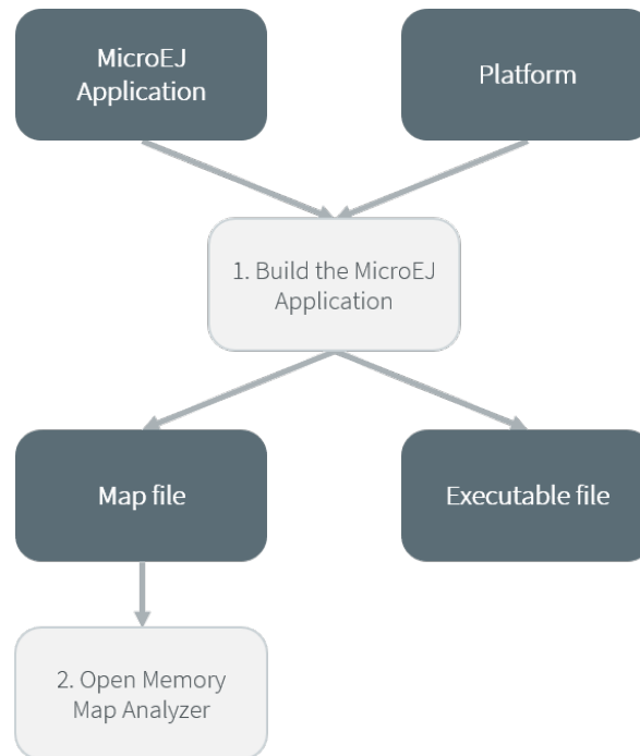
Fig. 64: Memory Map Analyzer Process
