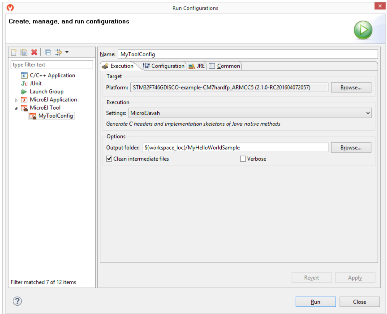
Fig. 34: MicroEJ Tool Configuration
