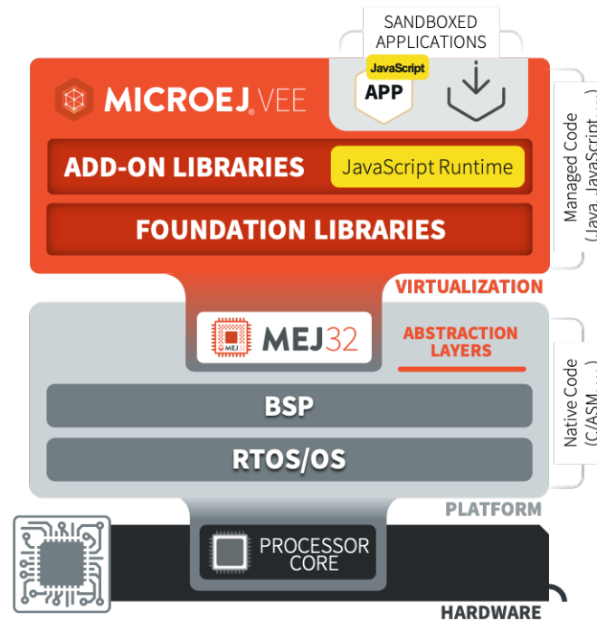
Fig. 77: MicroEJ JavaScript Overview
