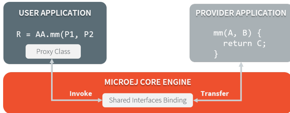
Fig. 19: Shared Interfaces Proxy Overview
