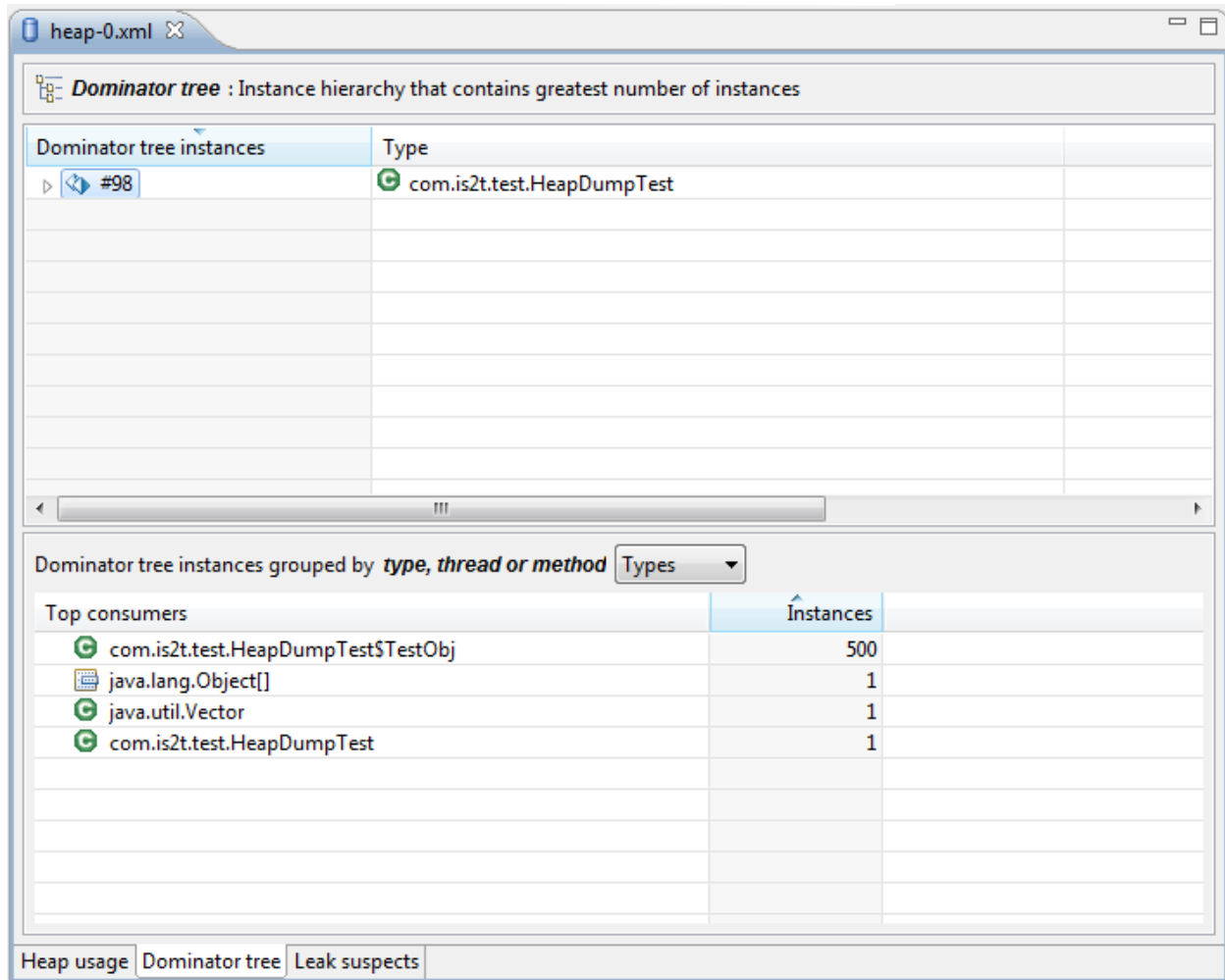
Fig. 58: Heap Viewer - Dominator Tree Tab
