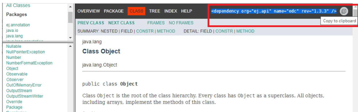
Fig. 23: Example of Javadoc Module Dependency
