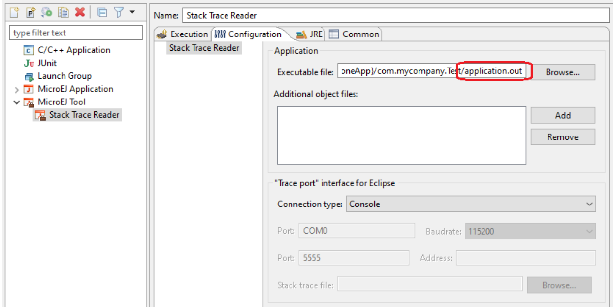
Fig. 42: Stack Trace Reader Tool Configuration (Standalone Application)
