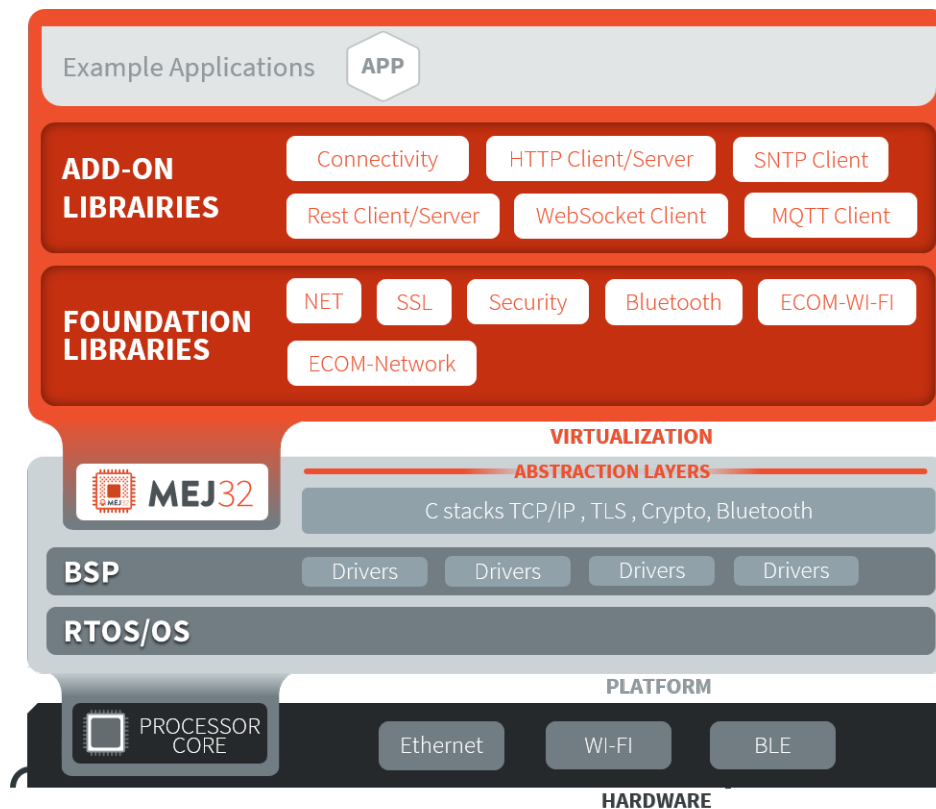
Fig. 72: Network Libraries Overview
