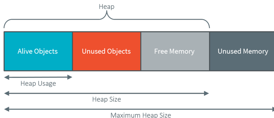
Fig. 48: Heap Structure Summary
