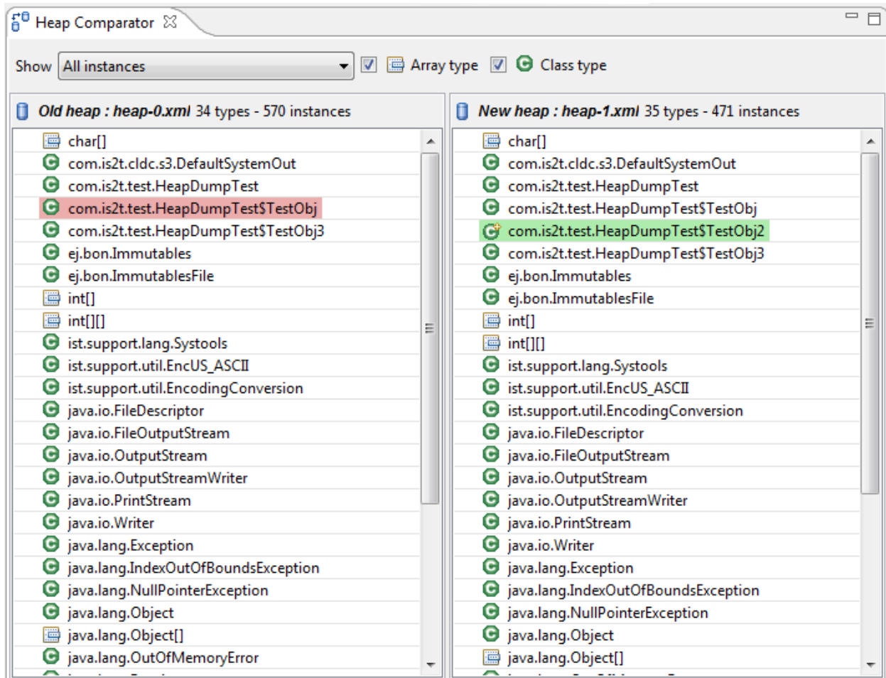
Fig. 56: Compare Heap Dumps
