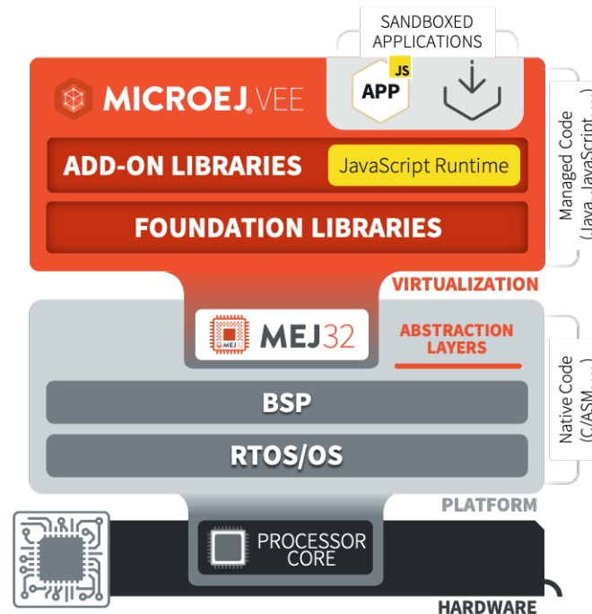
Fig. 71: MicroEJ JavaScript Overview
