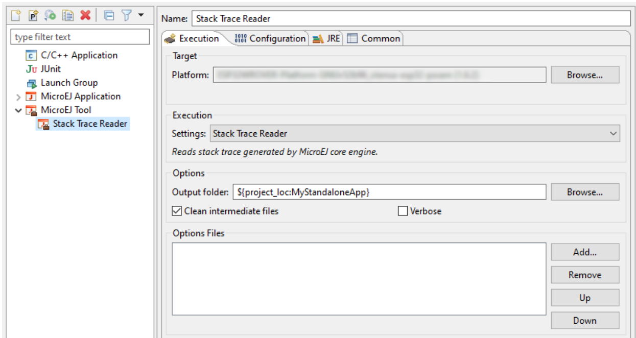
Fig. 36: Stack Trace Reader Tool Configuration (Platform Selection)
