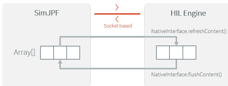
Fig. 51: An Array and Its Counterpart in the HIL Engine.
