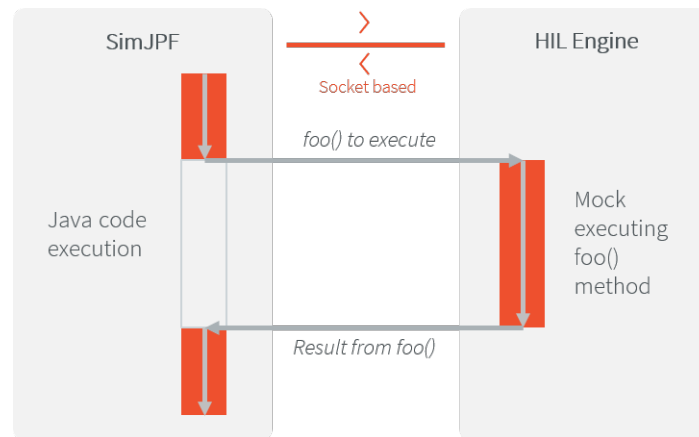
Fig. 50: The MicroEJ Simulator Executes a Native Java Method foo() .
