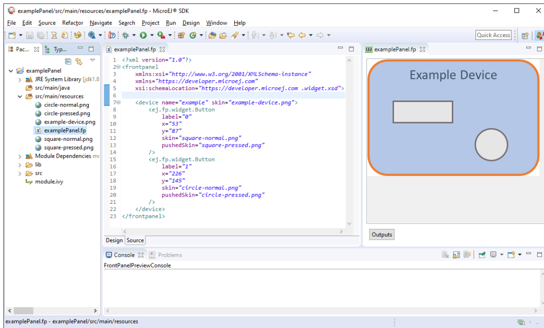
Fig. 55: Working Layout Example
