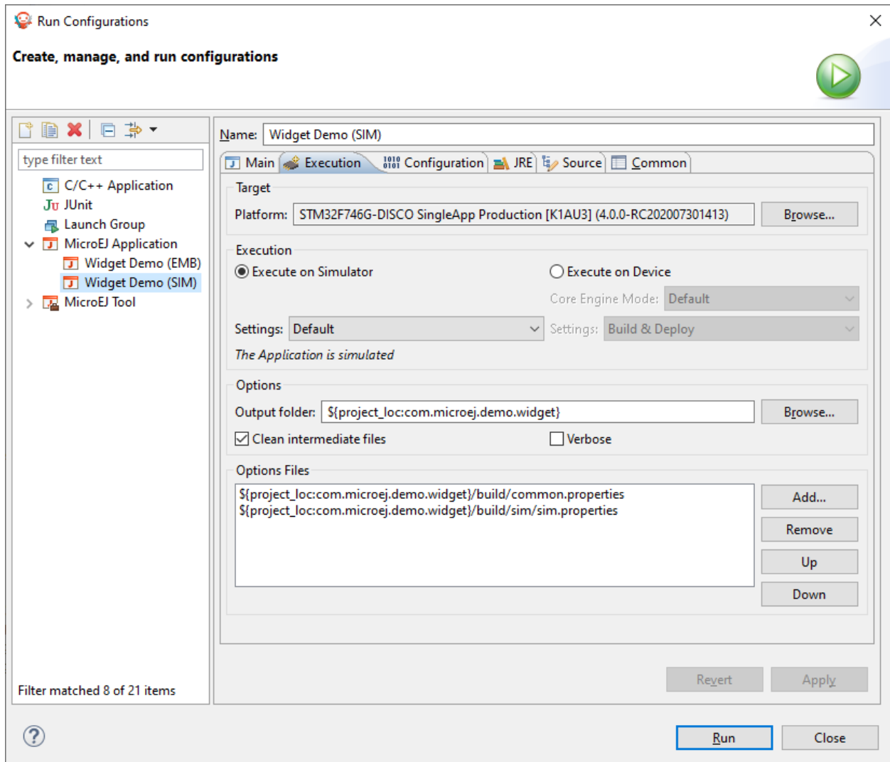
Fig. 18: MicroEJ Launch Application Execution Tab
