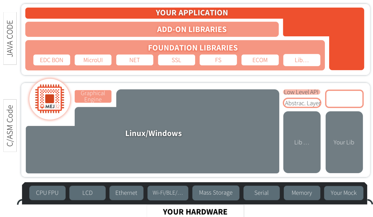
Fig. 24: MicroEJ Virtual Device Architecture
