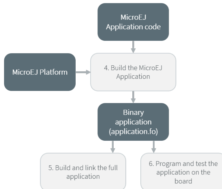
Fig. 15: Multi-Sandbox Process
