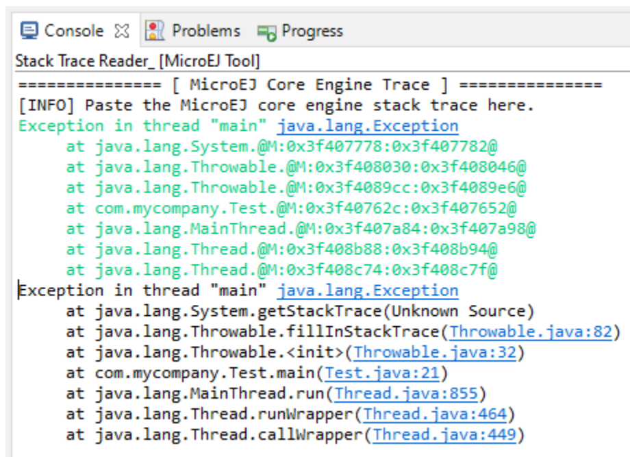
Fig. 40: Stack Trace Reader Console
