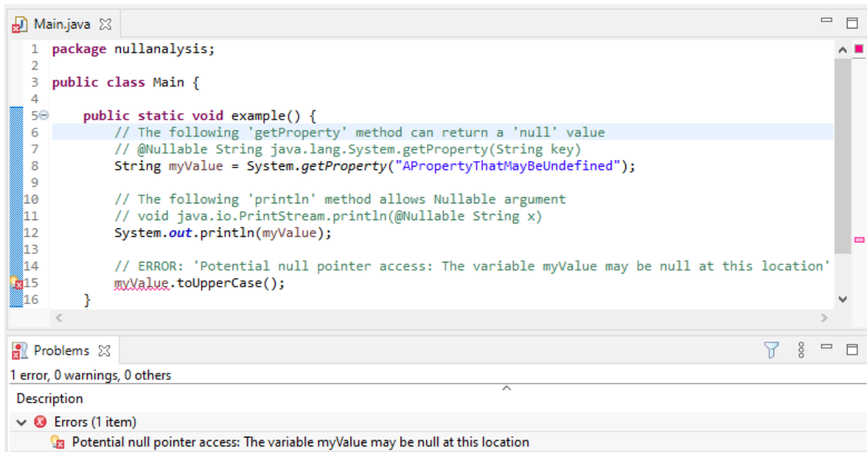
Fig. 65: Example of Null Analysis Detection
