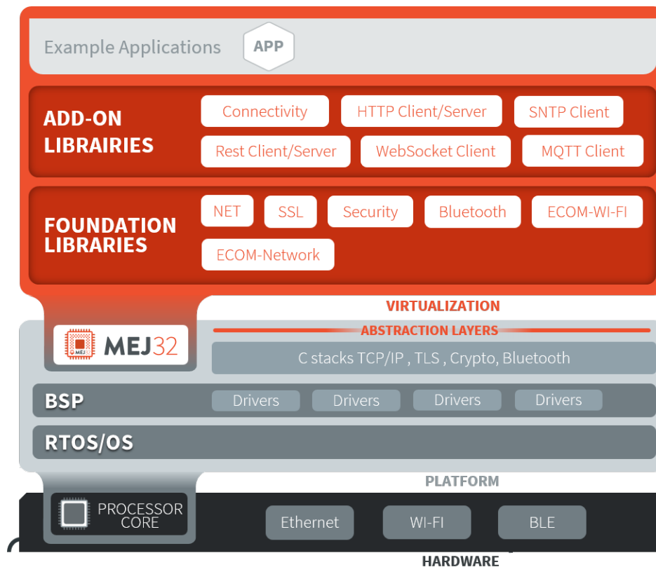
Fig. 74: Network Libraries Overview
