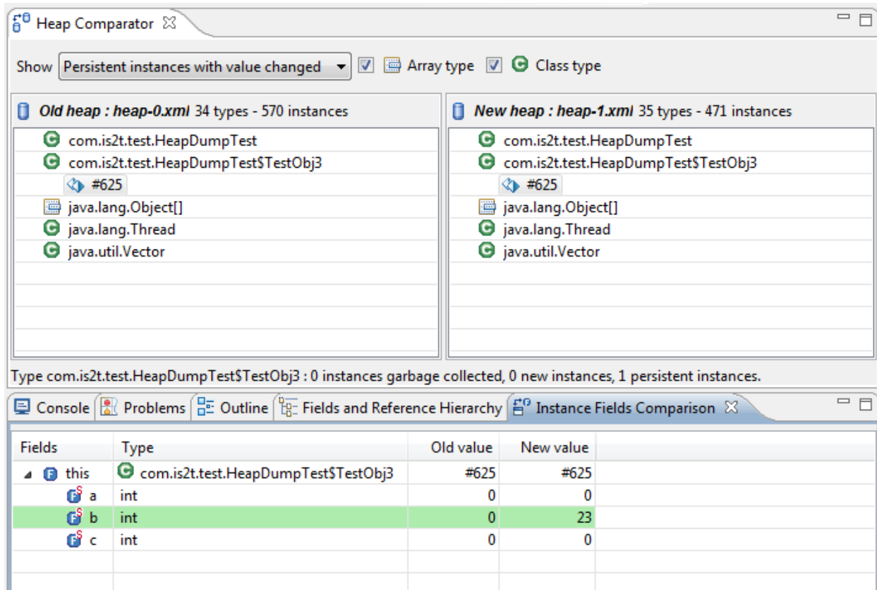
Fig. 59: Instance Fields Comparison view
