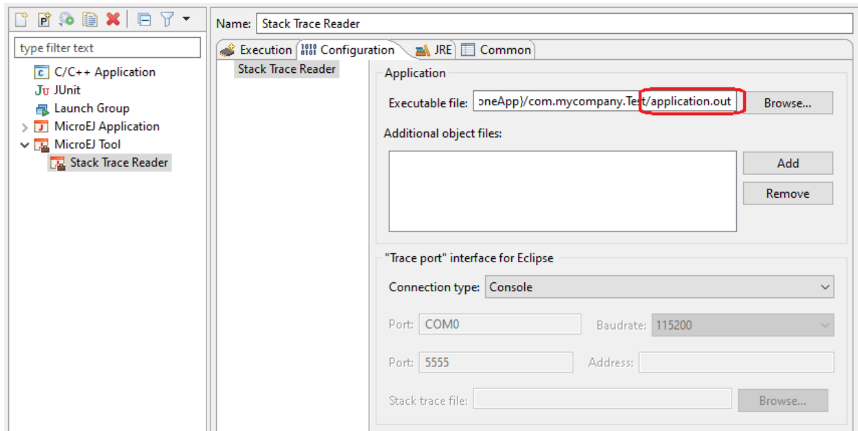
Fig. 39: Stack Trace Reader Tool Configuration (Standalone Application)
