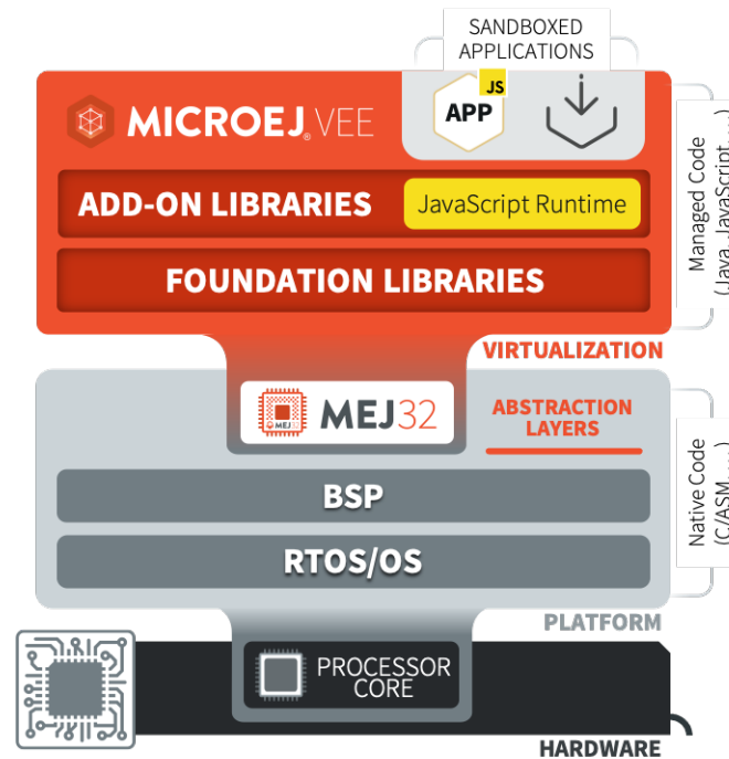
Fig. 73: MicroEJ JavaScript Overview
