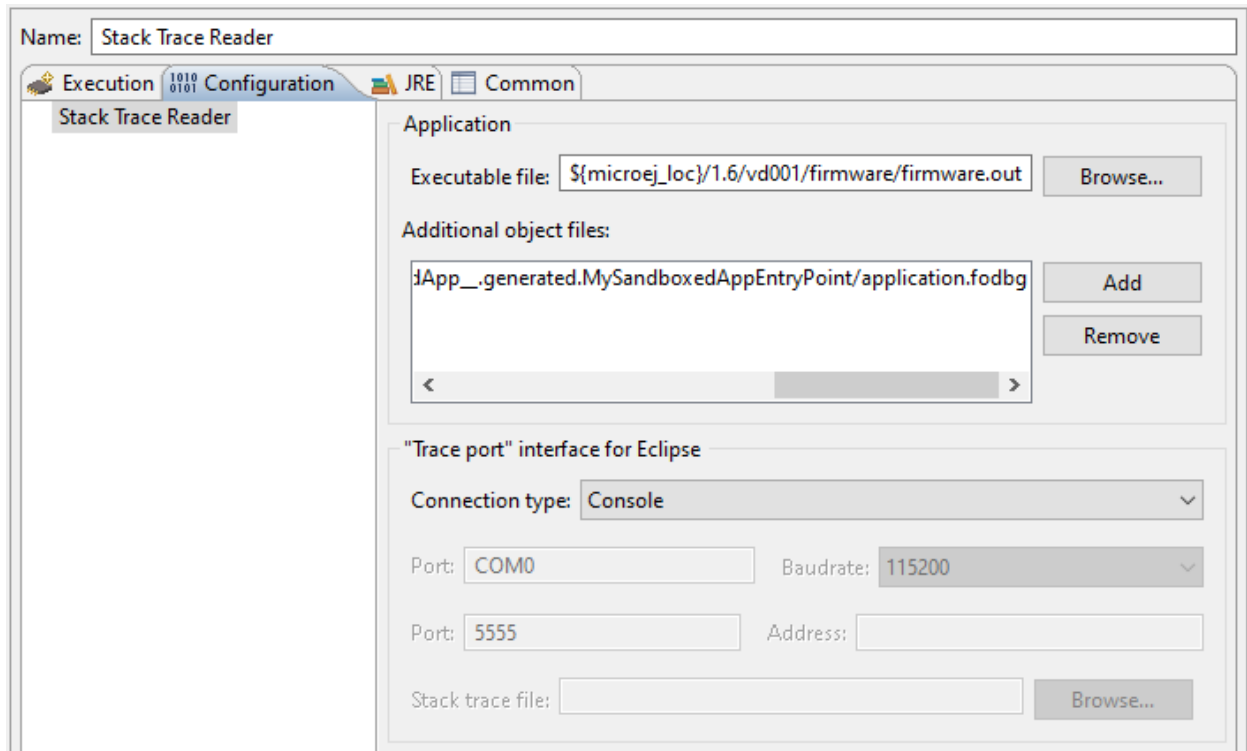
Fig. 45: Select the Kernel Executable File
