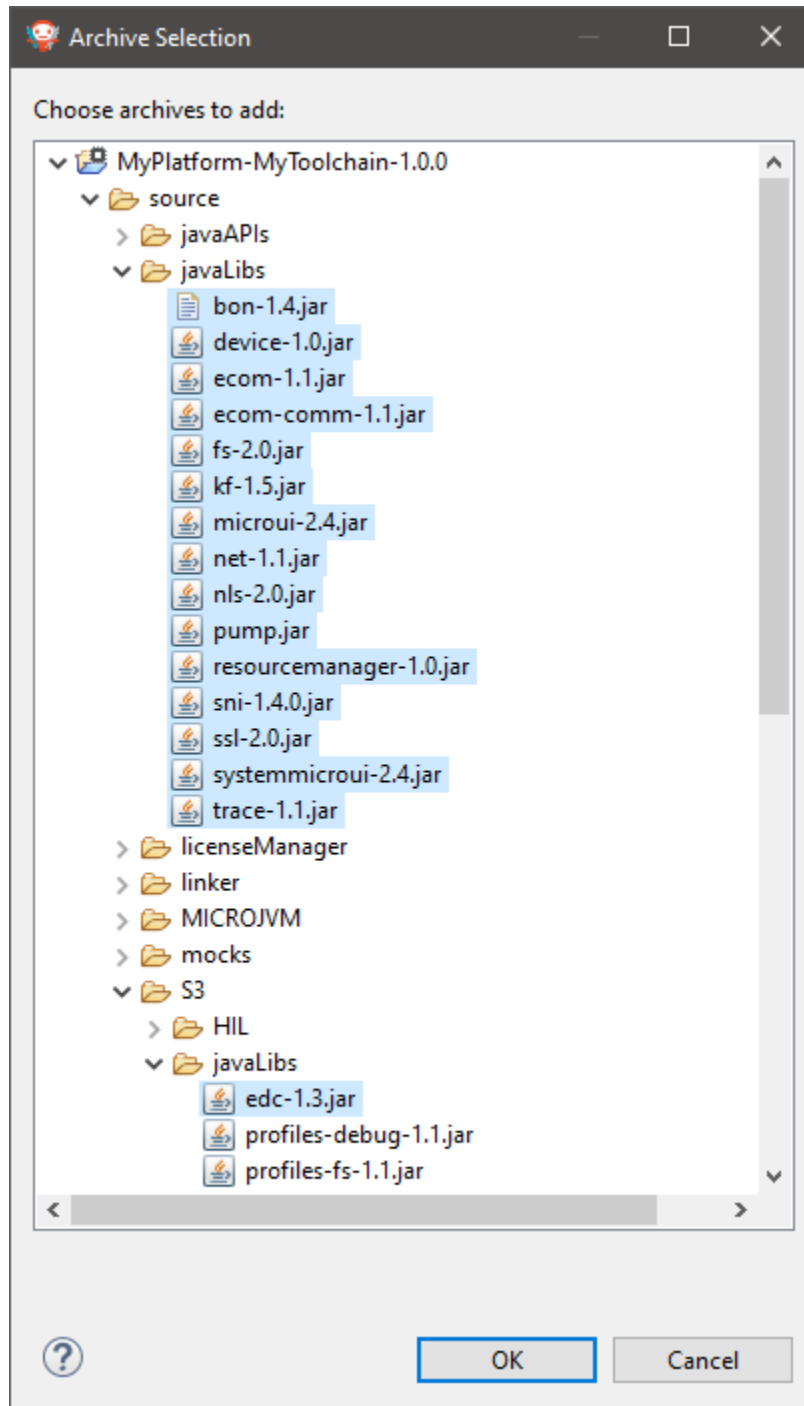
Fig. 29: Select Foundation Libraries Implementation files
