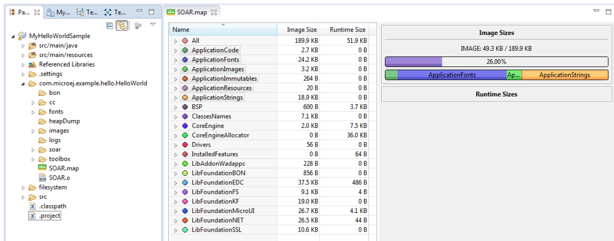
Fig. 63: Consult Full Memory
