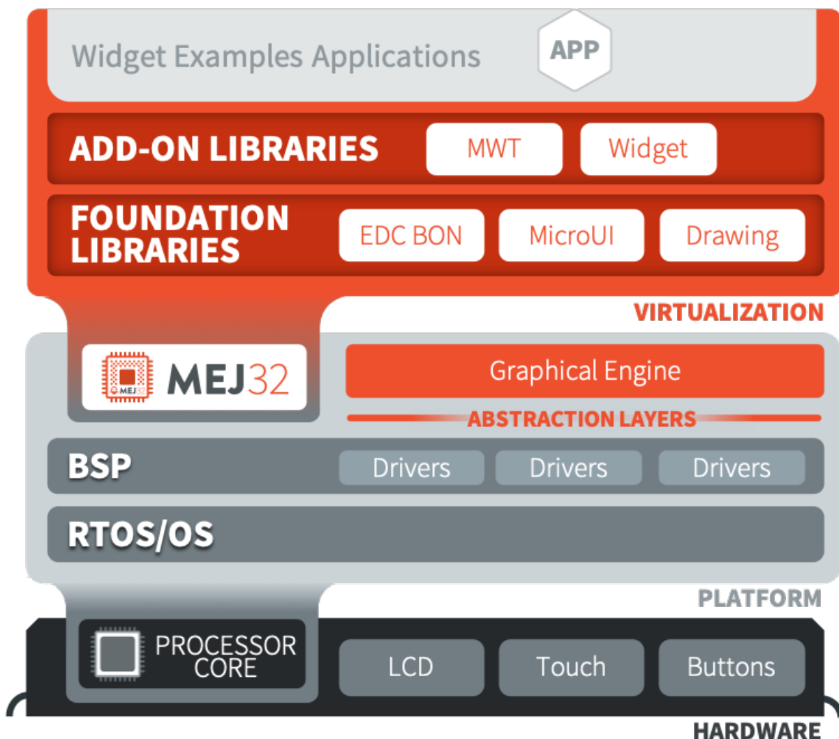
Fig. 67: Graphical User Interface Overview
