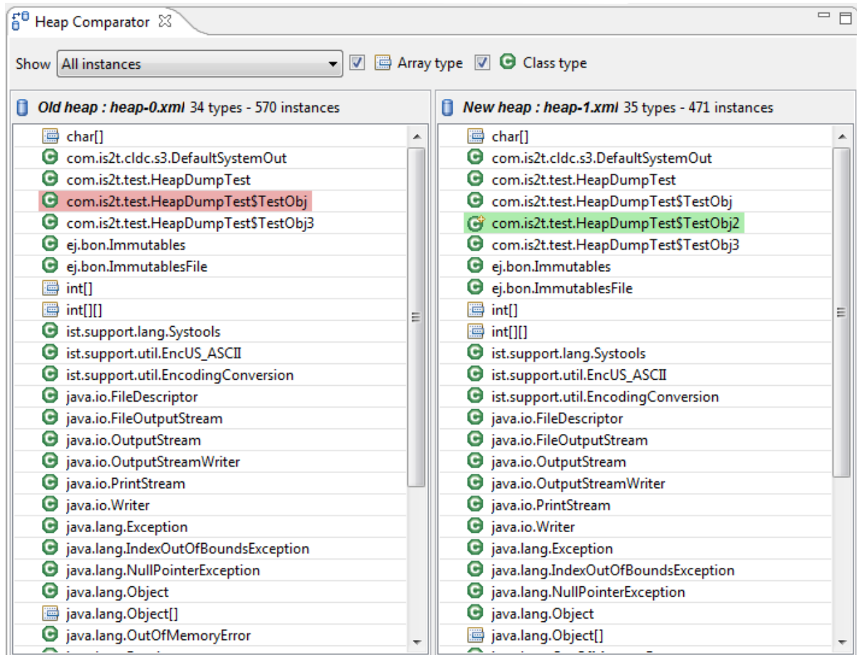
Fig. 58: Compare Heap Dumps
