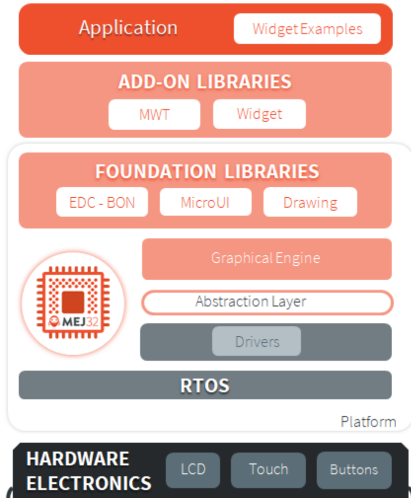
Fig. 53: Graphics User Interface Overview
