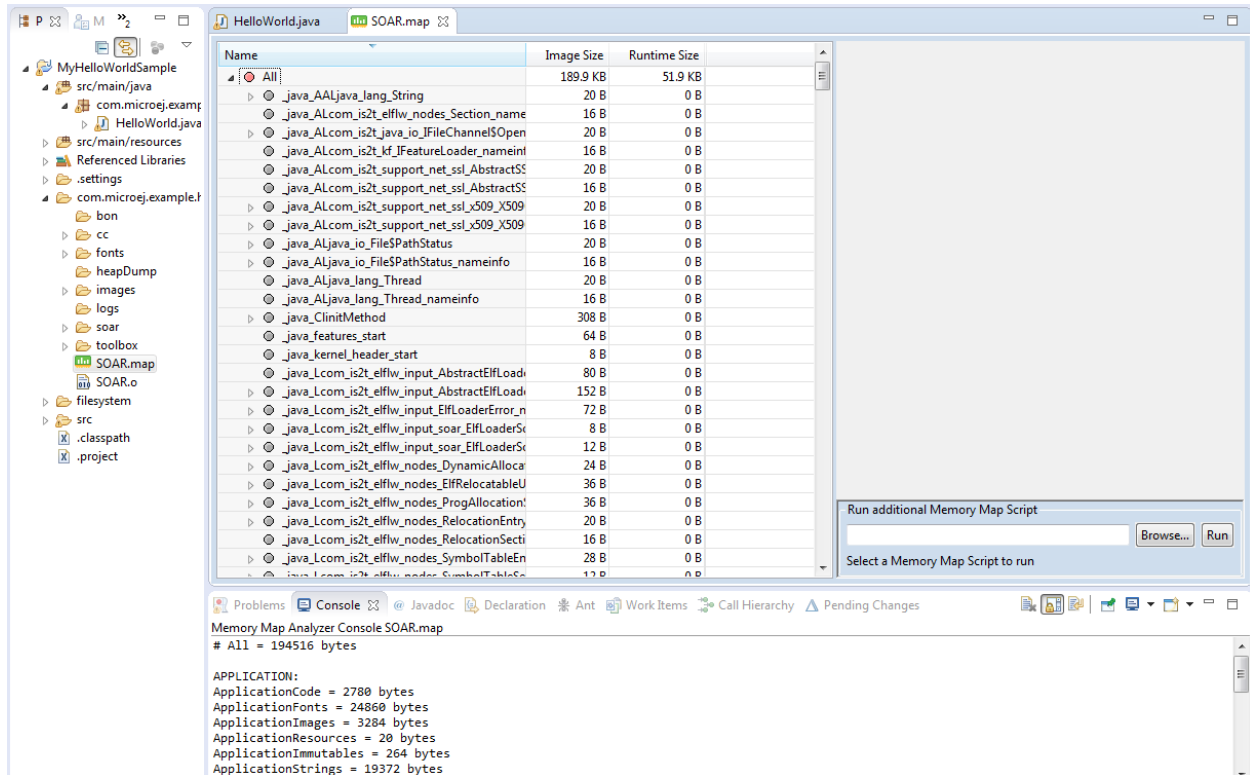
Fig. 52: Detailed View
