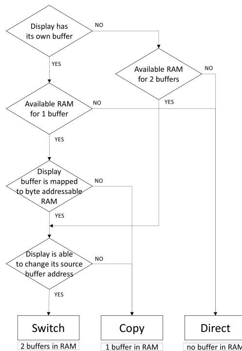
Fig. 35: Buffer Modes
