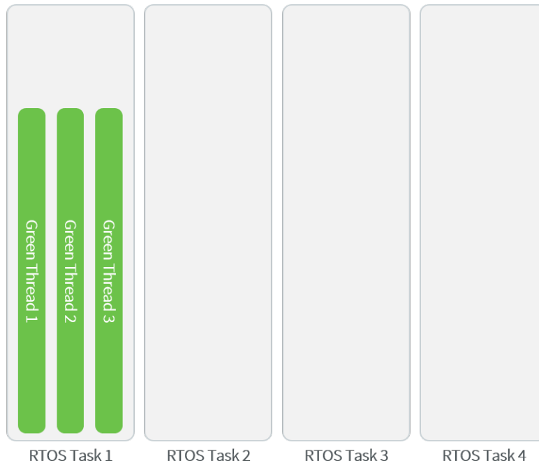
Fig. 20: A Green Threads Architecture Example
