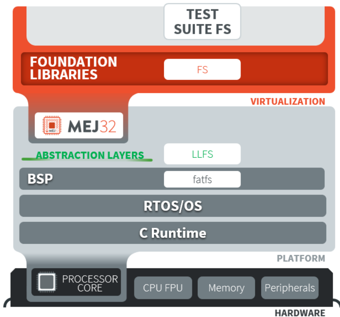
Fig. 15: Platform Qualification Example for FS Pack
