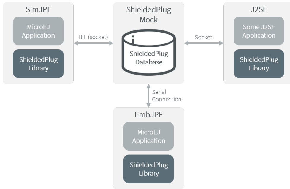
Fig. 51: Shielded Plug Mock General Architecture
