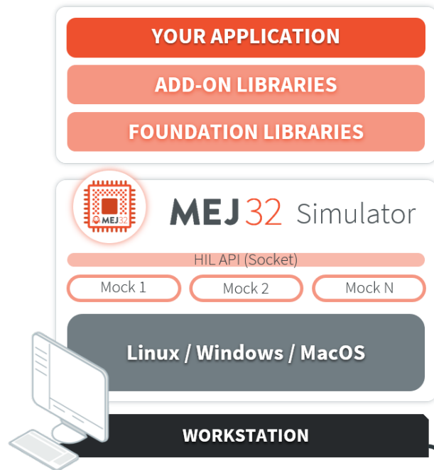
Fig. 47: The HIL Connects the MicroEJ Simulator to the Workstation.
