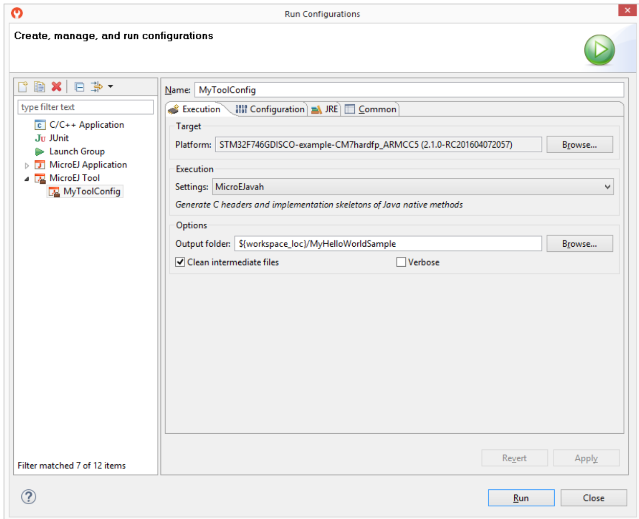
Fig. 26: MicroEJ Tool Configuration
