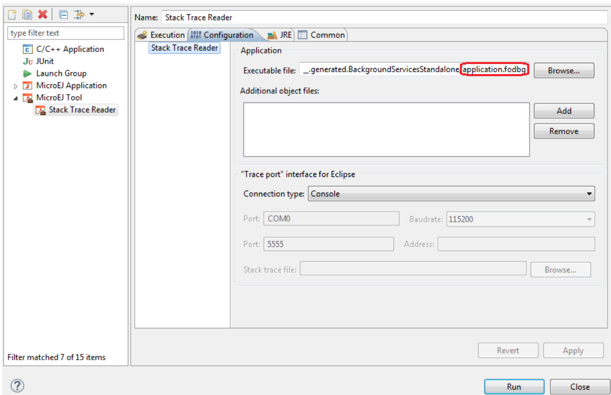
Fig. 35: Stack Trace Reader Tool Configuration (Sandboxed Application)
