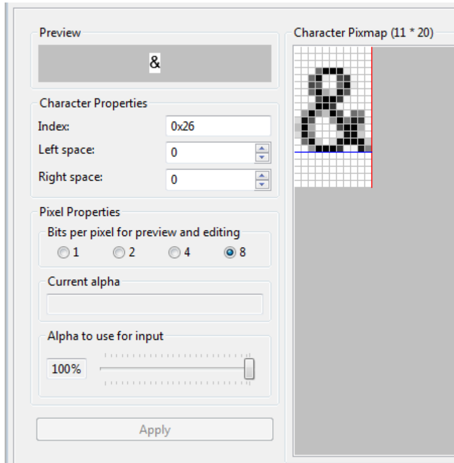
Fig. 57: Character Editor
