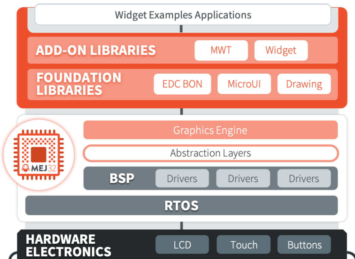
Fig. 53: Graphical User Interface Overview
