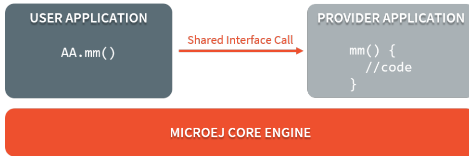
Fig. 15: Shared Interface Call Mechanism
