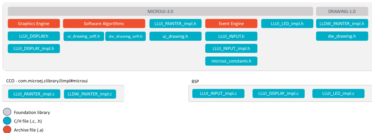
Fig. 33: MicroUI Embedded Low Level API
