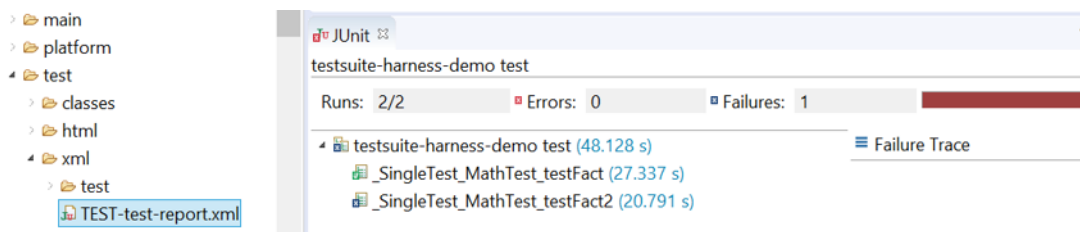
Fig. 27: Example of MicroEJ Test Suite XML Report in JUnit View
