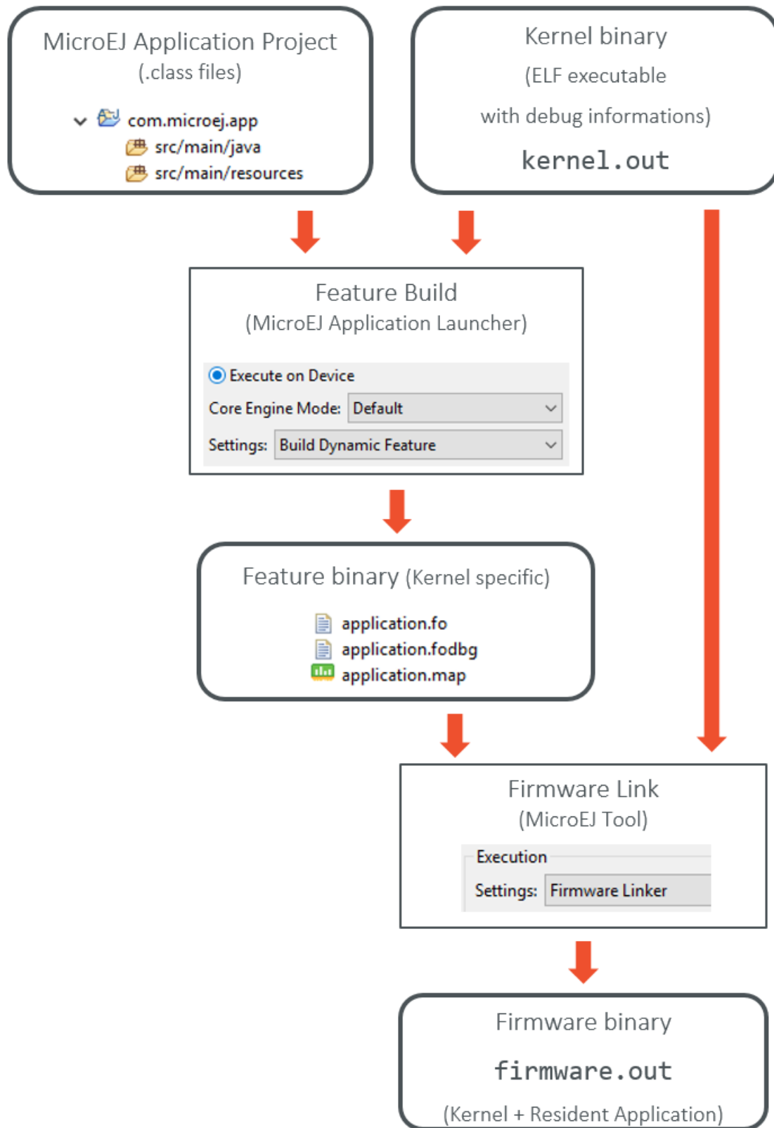
Fig. 6: Firmware Build Flow using MicroEJ Launches
