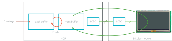
Fig. 65: Swap Double Buffer
