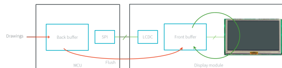
Fig. 63: Single Buffer (serial)
