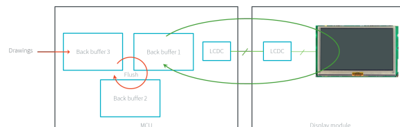
Fig. 66: Swap Triple Buffer
