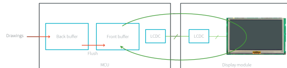
Fig. 59: Single Buffer (parallel)
