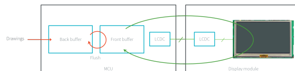
Fig. 56: Swap Double Buffer
