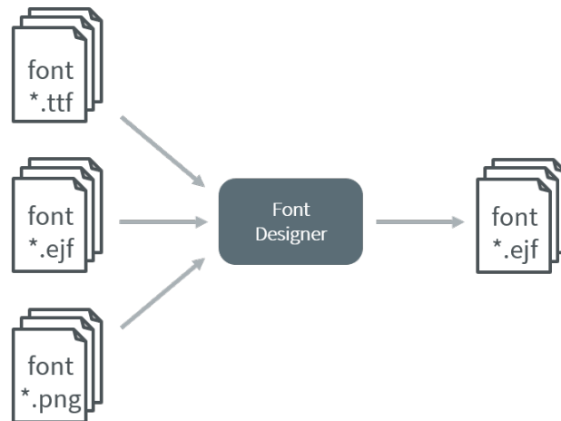
Fig. 53: Font Generation
