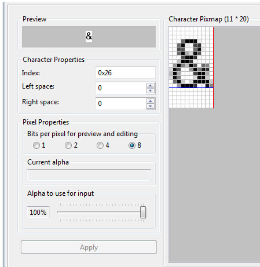
Fig. 73: Character Editor
