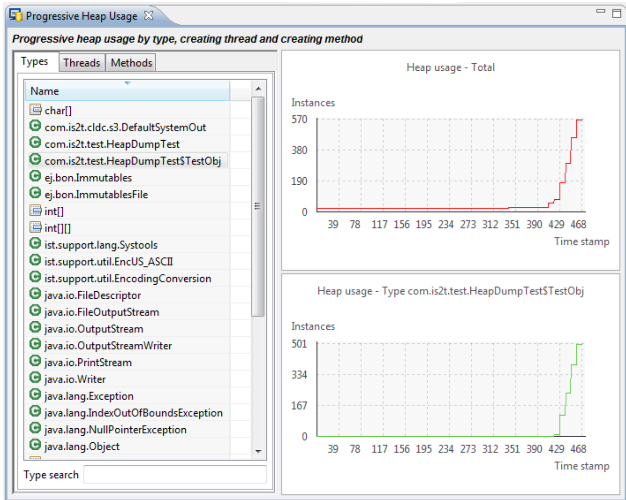
Fig. 54: Progressive Heap Usage
