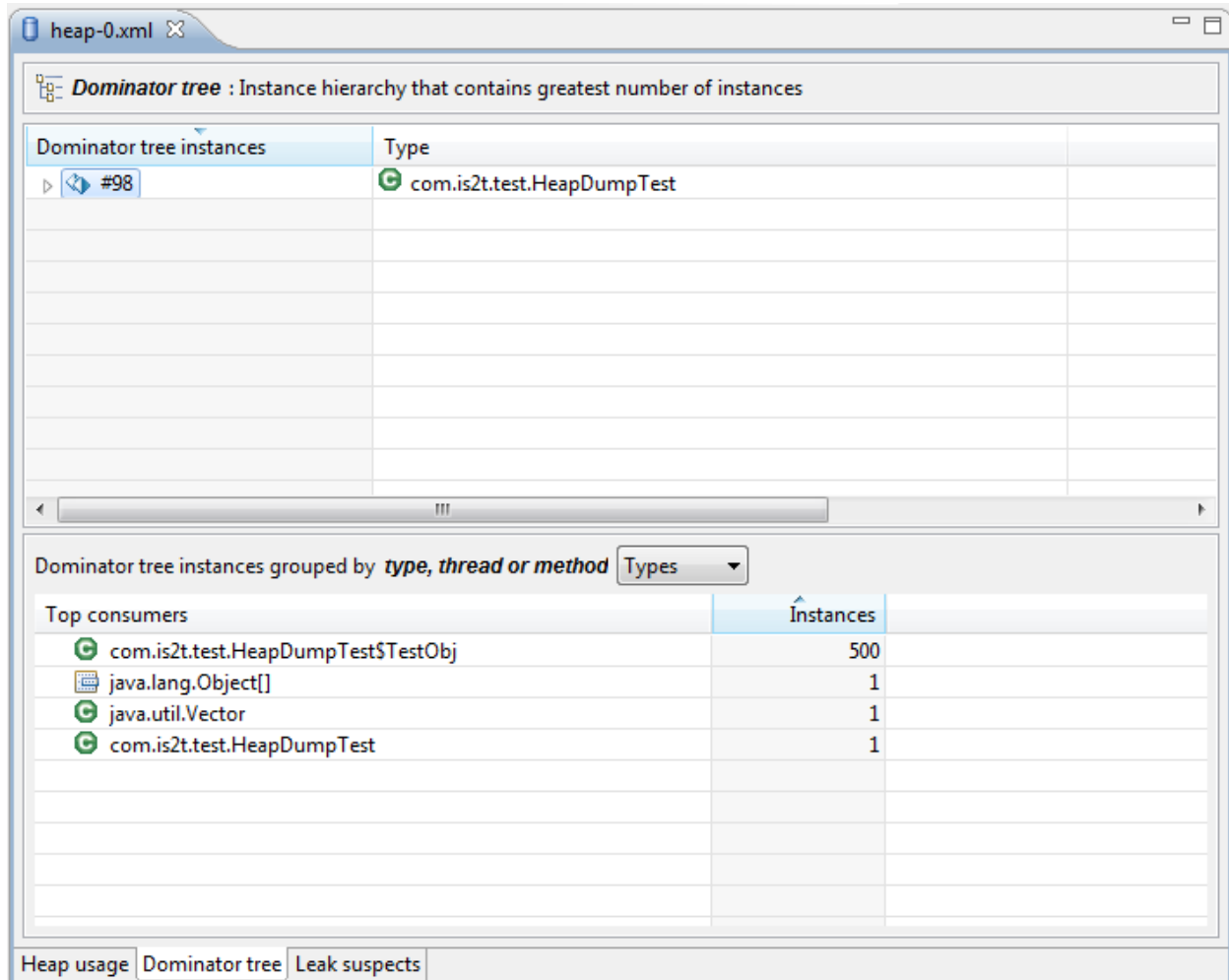
Fig. 52: Heap Viewer - Dominator Tree Tab
