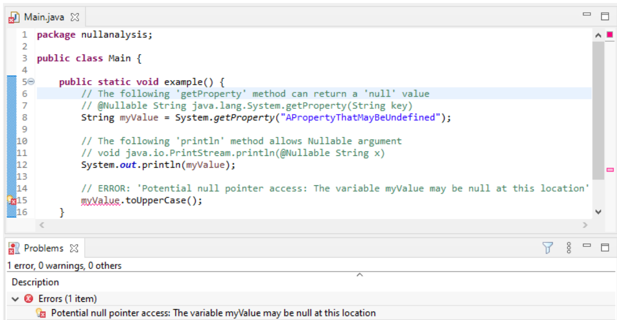
Fig. 62: Example of Null Analysis Detection
