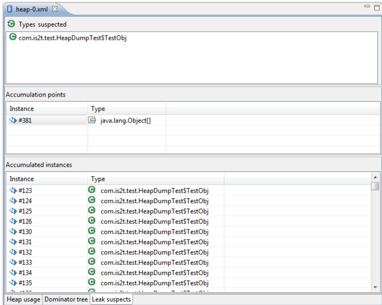
Fig. 53: Heap Viewer - Leak Suspects Tab
