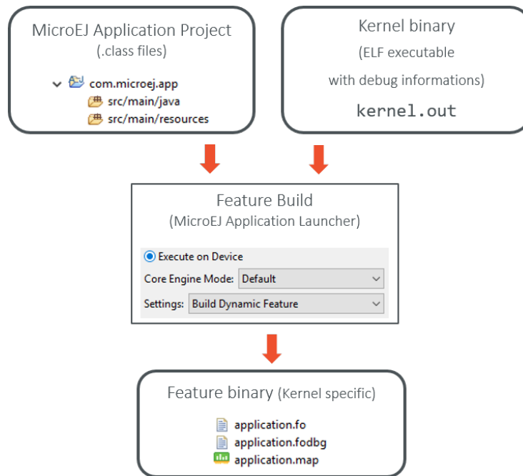
Fig. 13: Feature Build Flow using MicroEJ Launch
