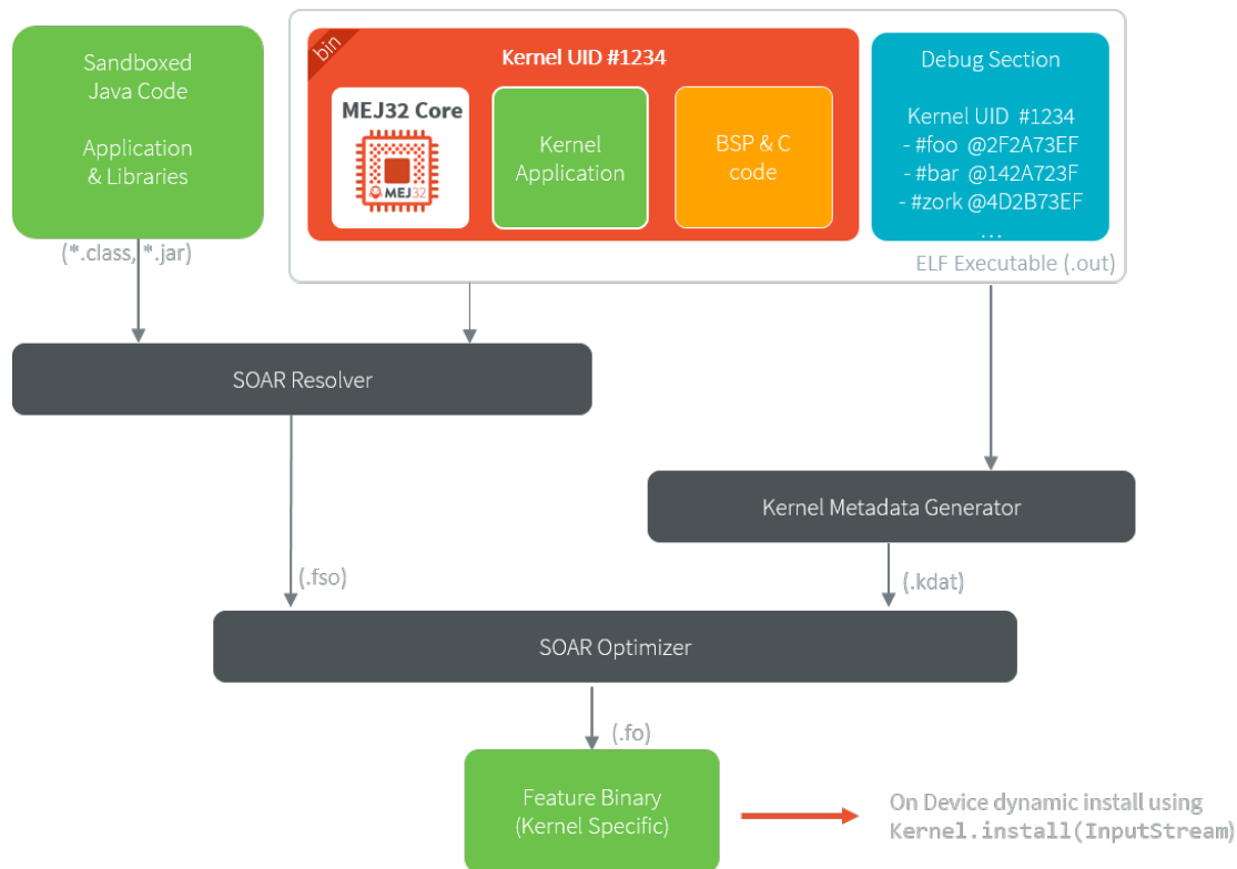
Fig. 12: Sandboxed Application Build Flow
