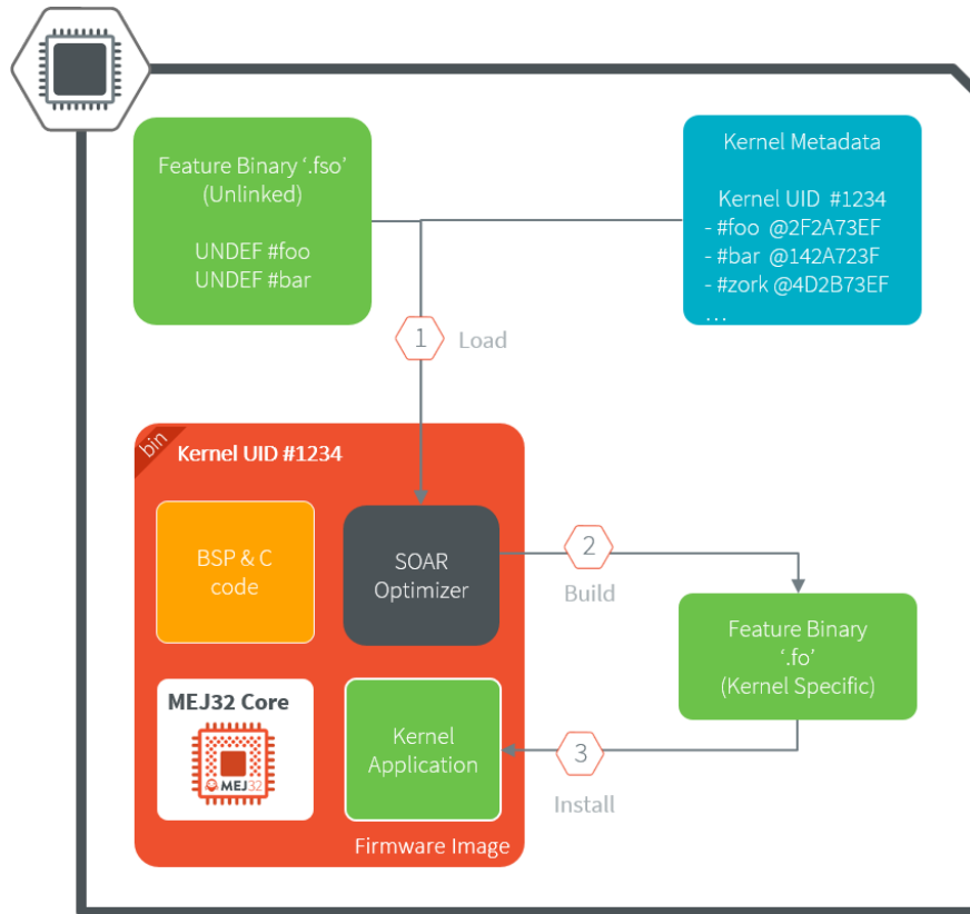
Fig. 14: Sandboxed Application Build on Device
