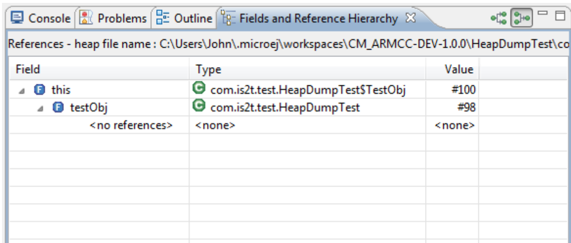
Fig. 56: Instance Browser View - References mode
