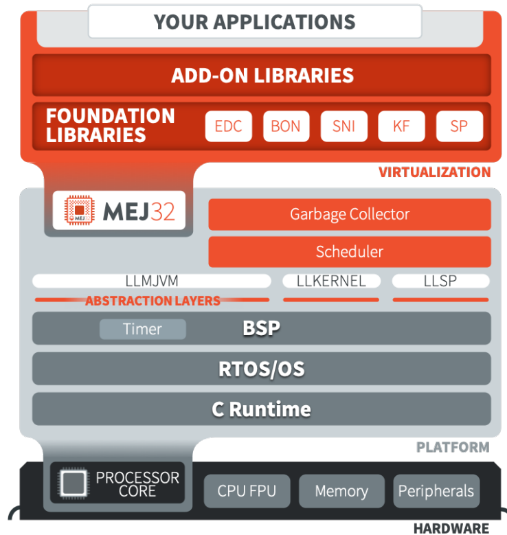
Fig. 1: MicroEJ Architecture Runtime Modules: Tools, Libraries and APIs
