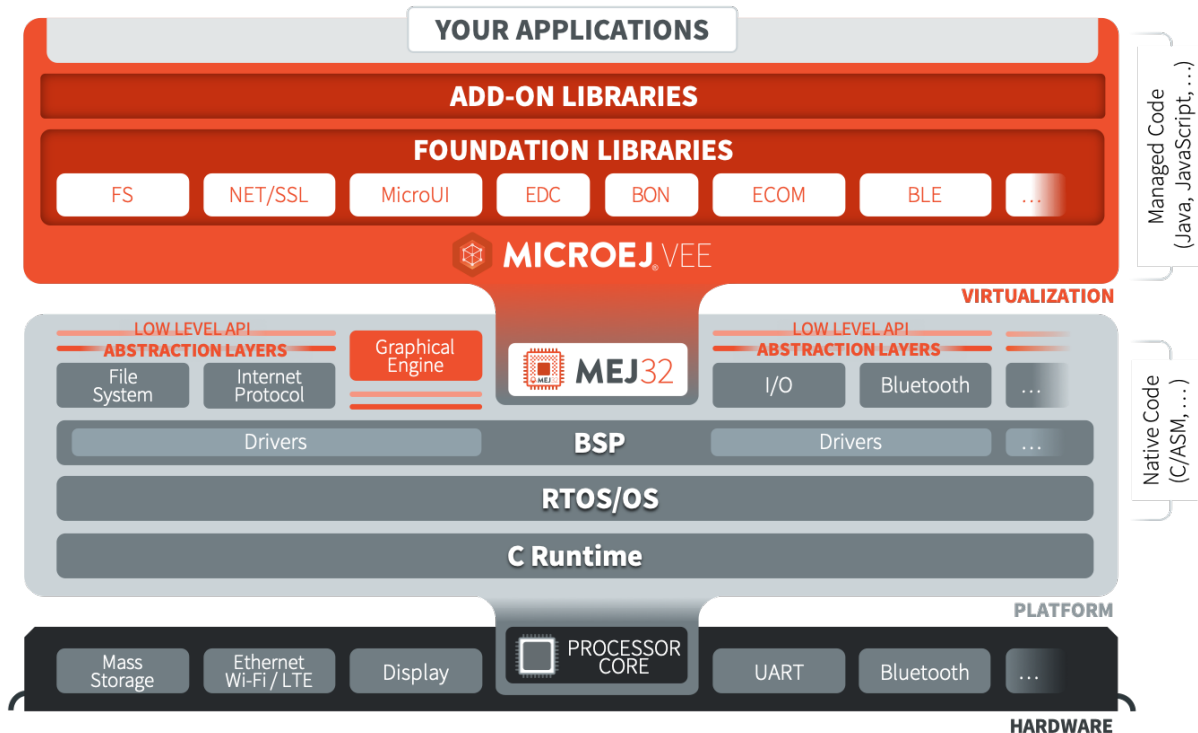
Fig. 10: MicroEJ Firmware Architecture
