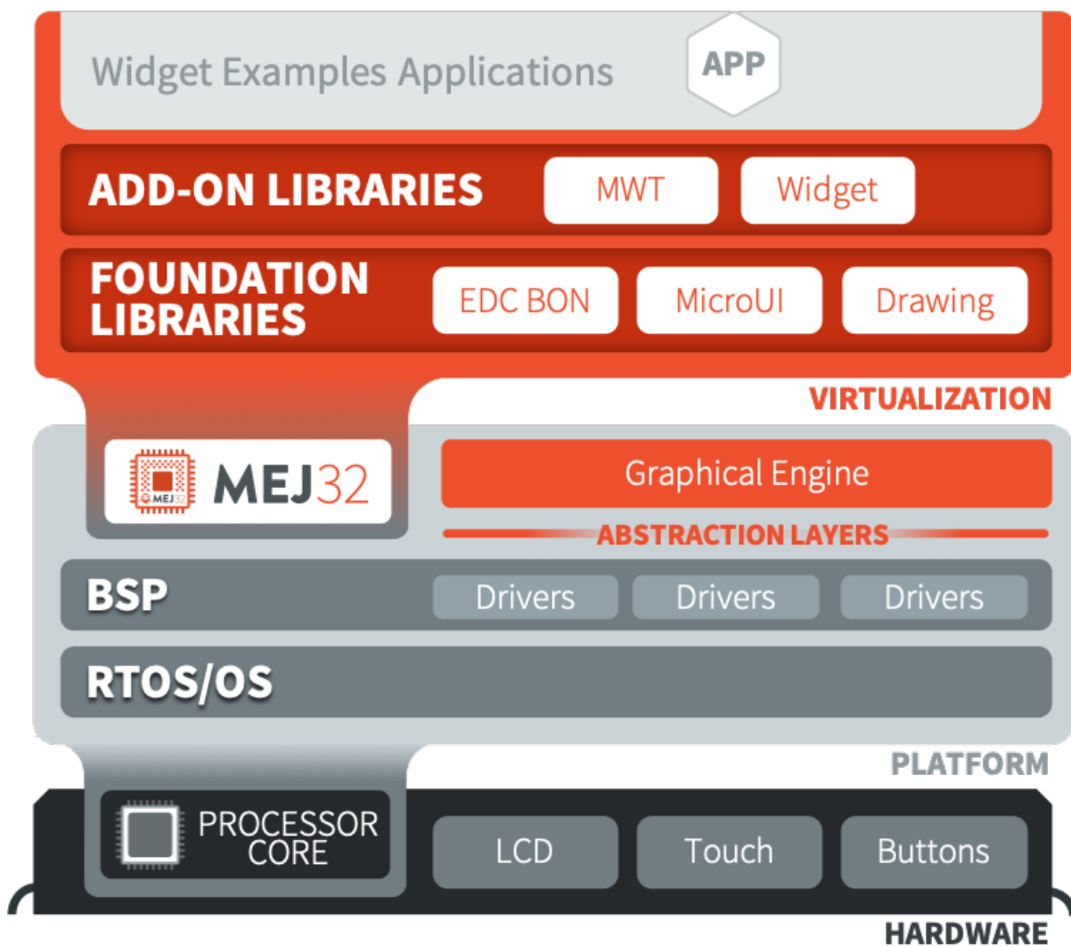
Fig. 55: Graphical User Interface Overview
