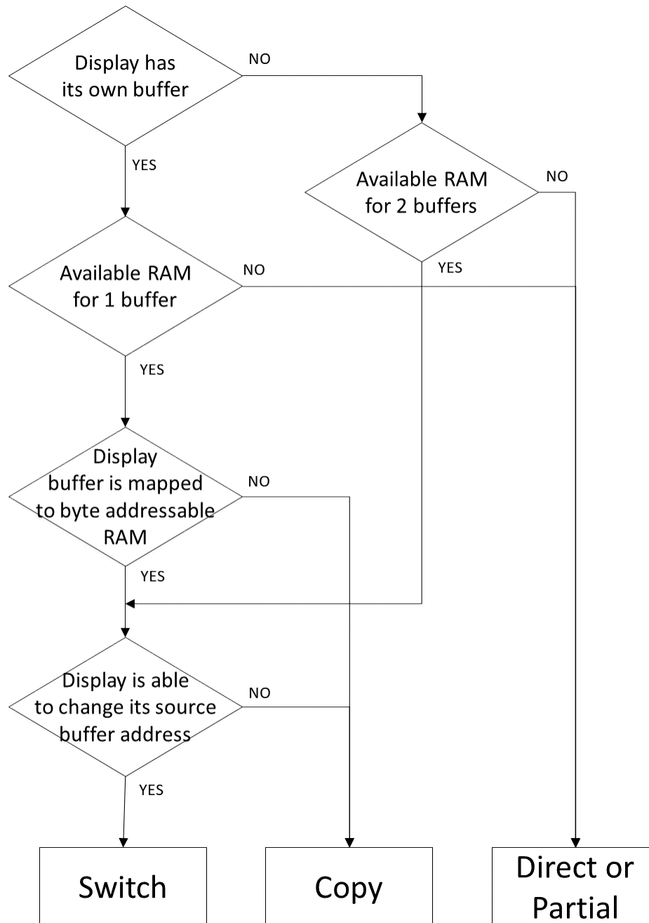
Fig. 36: Buffer Modes
