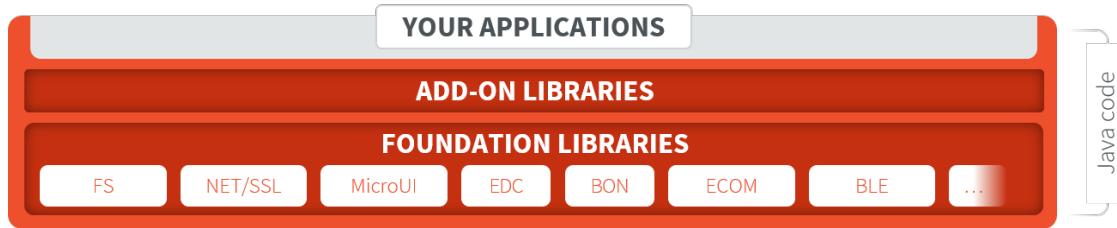
Fig. 9: MicroEJ Foundation Libraries and Add-On Libraries
