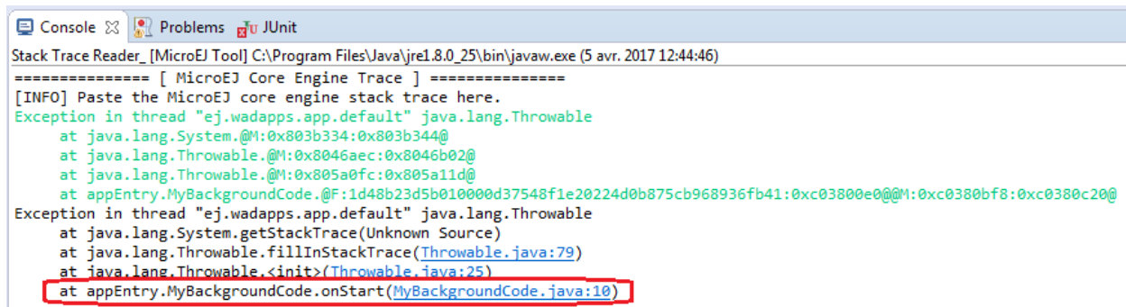
Fig. 39: Read the Stack Trace
